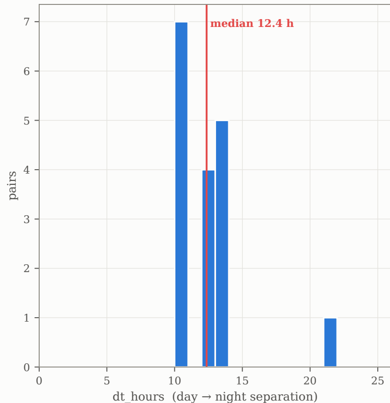
upper bound is next-day solar noon, not a fixed dt
