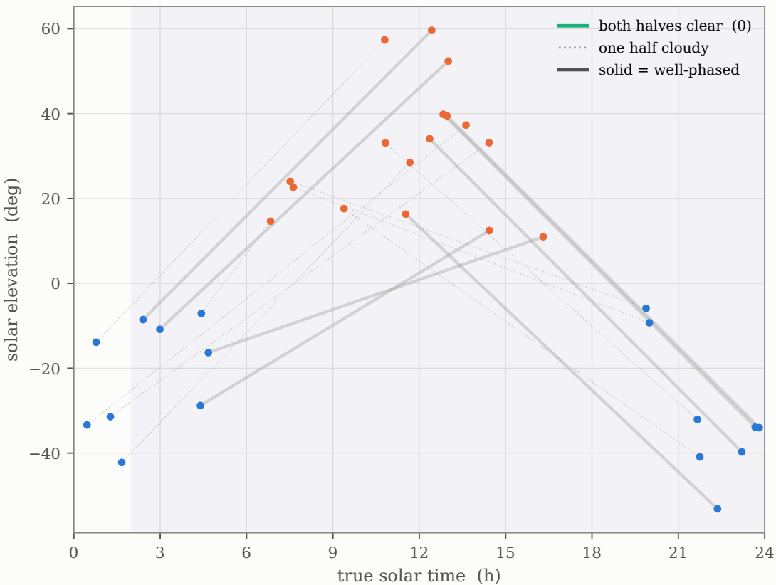
PSA2Tiergarten — each candidate pair, day half → night half
