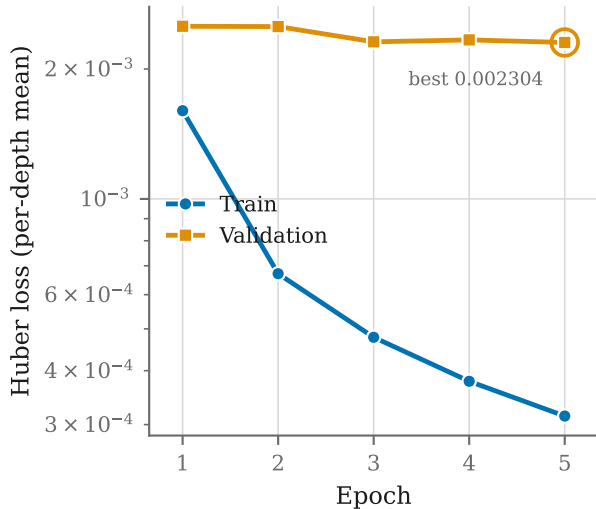
(a) Train vs. validation loss
