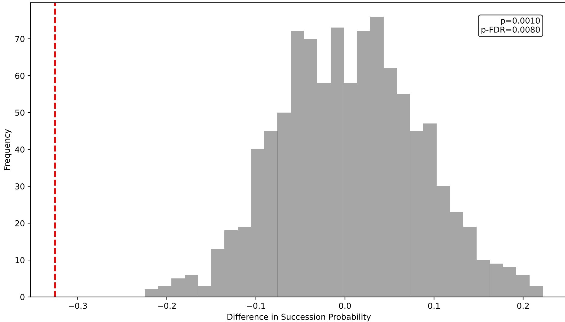
7-Network, k=4: Permutation Distribution - From S2 to S3
