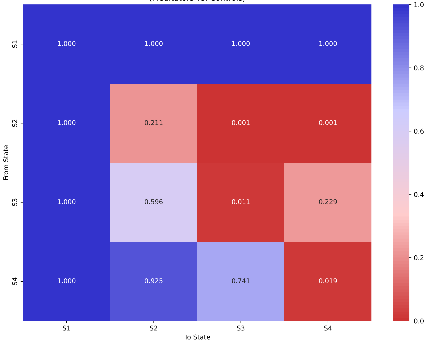
7-Network Configuration, k=4 Uncorrected P-values for State Succession Differences (Meditators vs. Controls)
