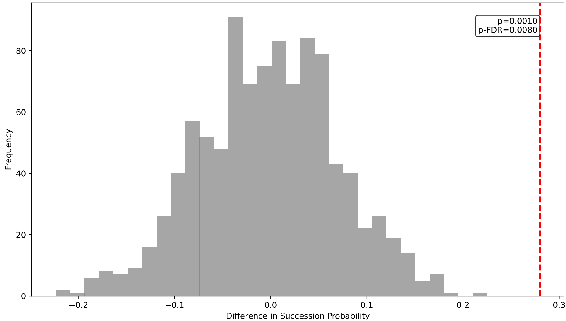
7-Network, k=4: Permutation Distribution - From S2 to S4
