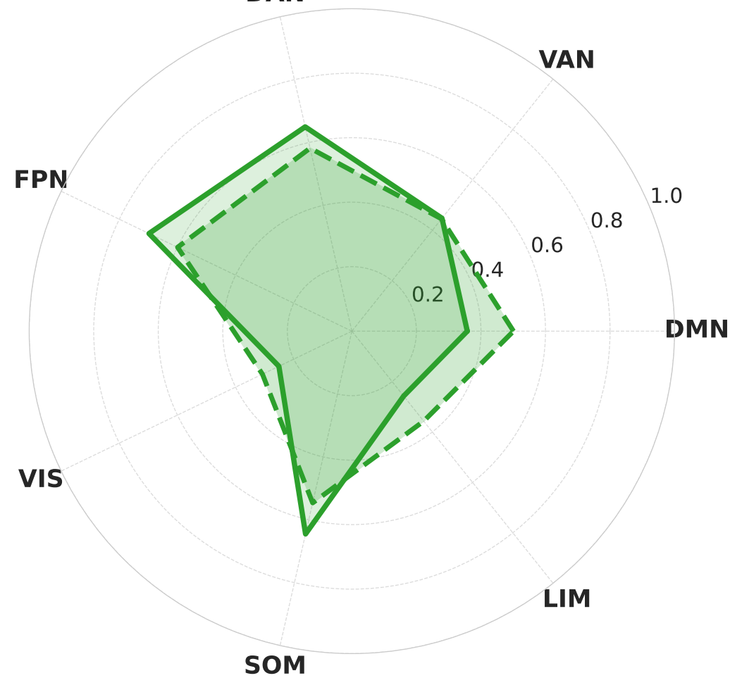
Breath Focus DAN
