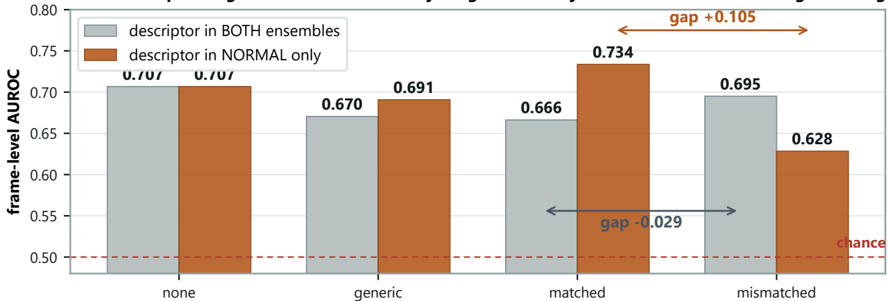
Context sweep, ShanghaiTech, w = 31 — everything frozen; only the sentence and where it goes change
