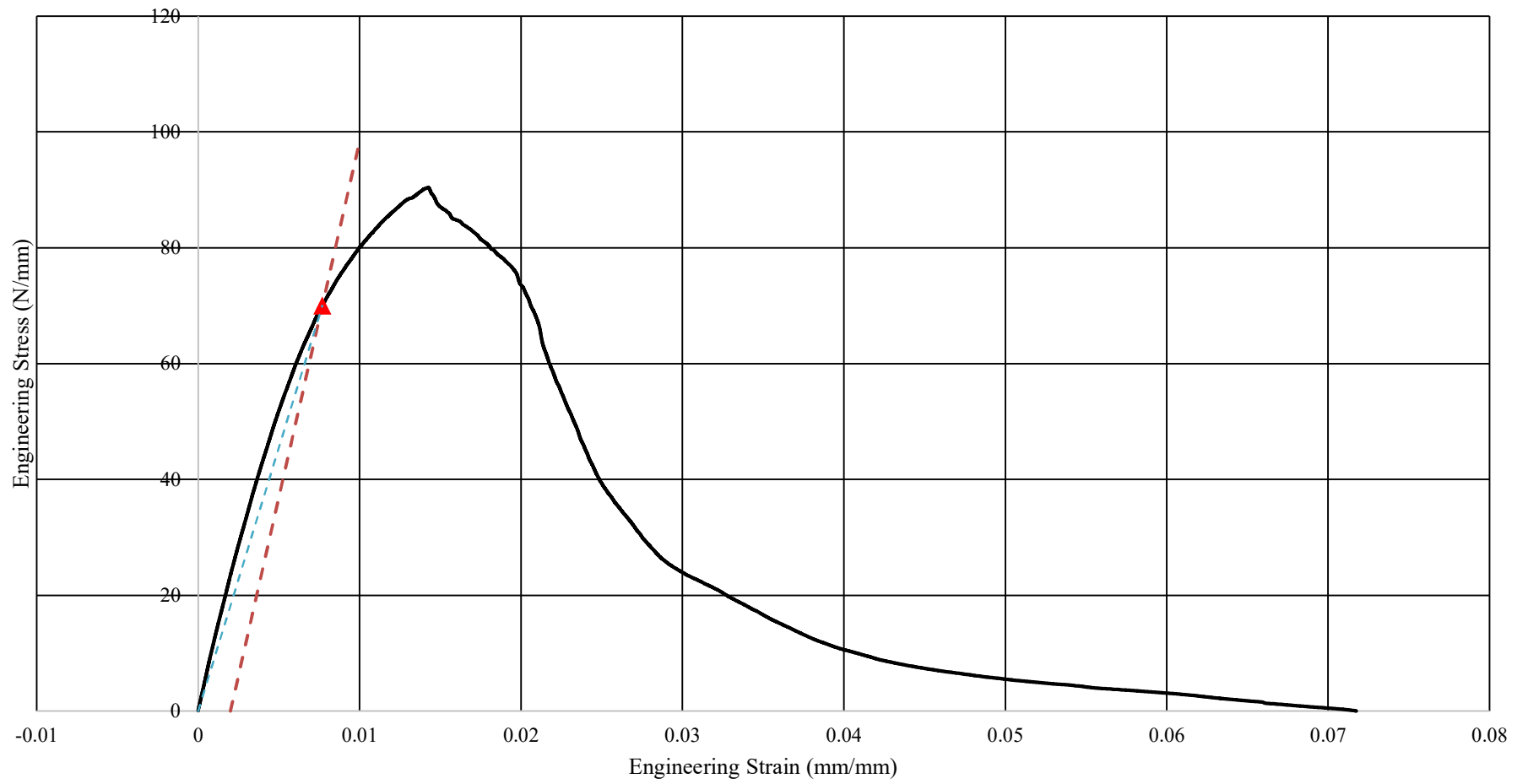
Engg. Stress Strain Curve
