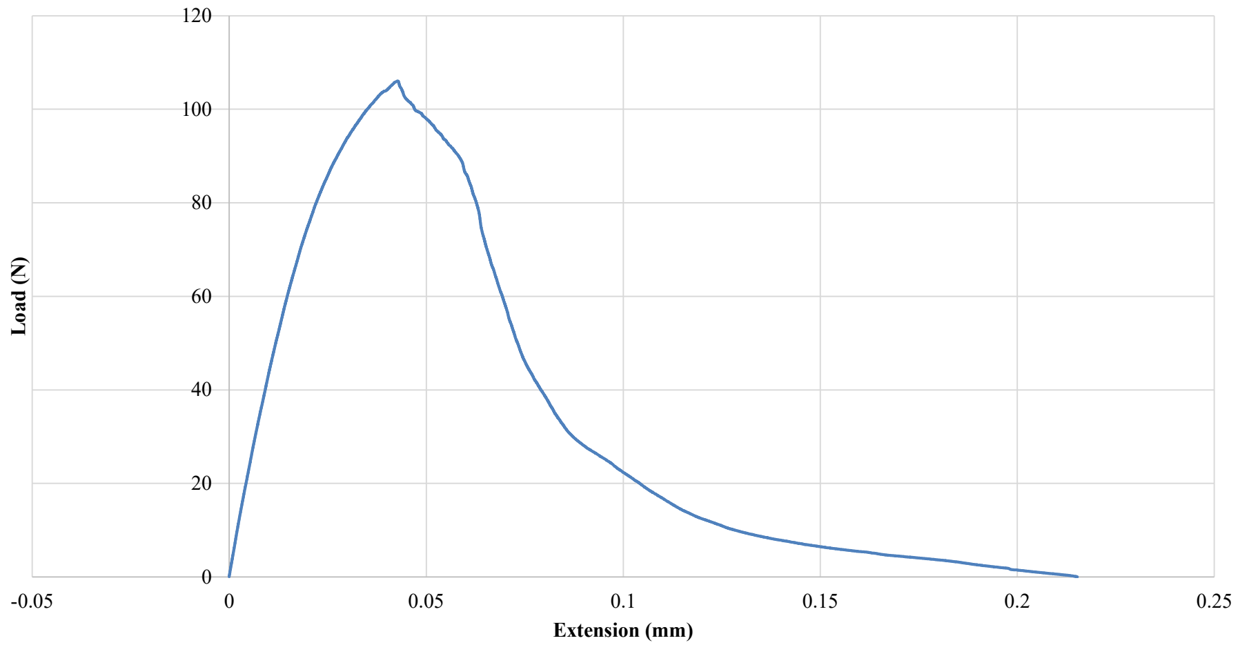
Load vs Extension Graph
