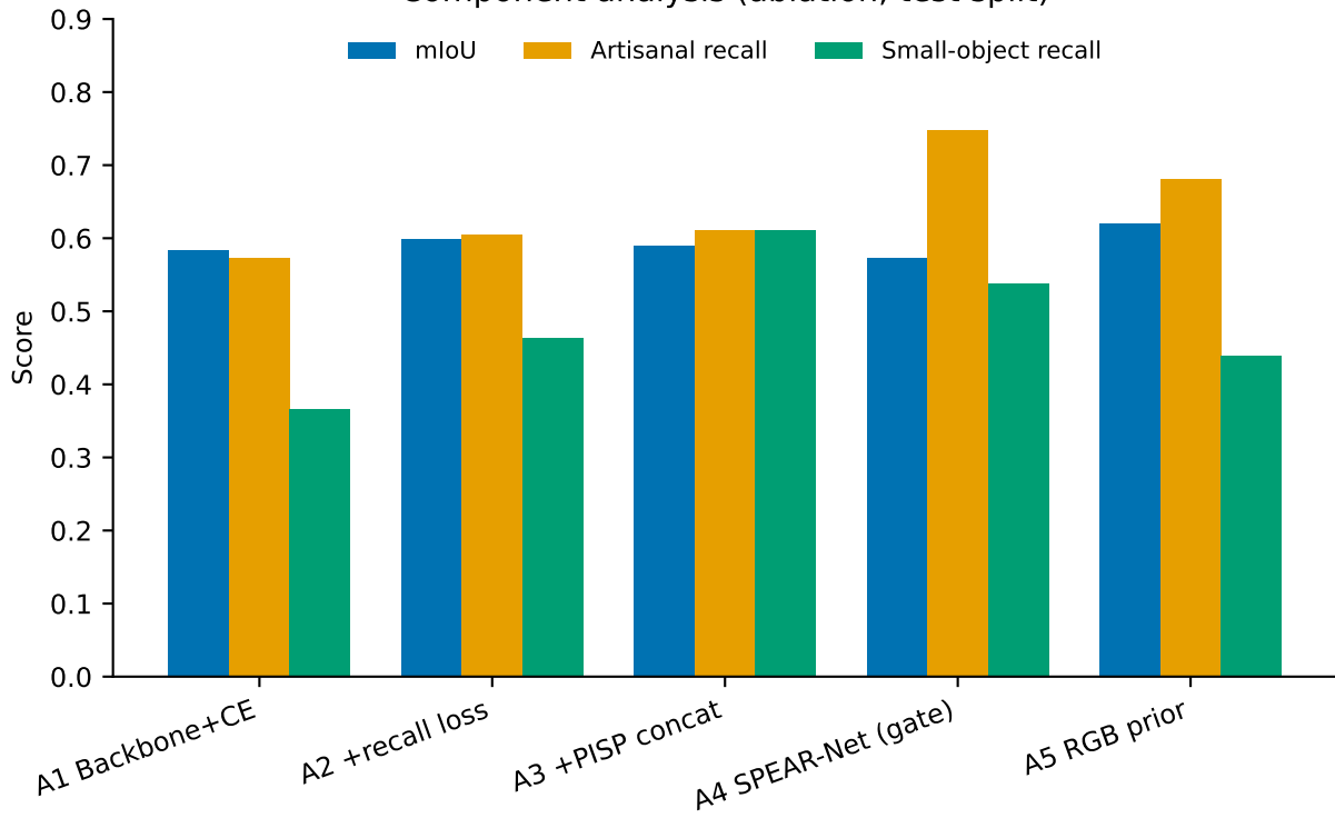
Component analysis (ablation, test split)
