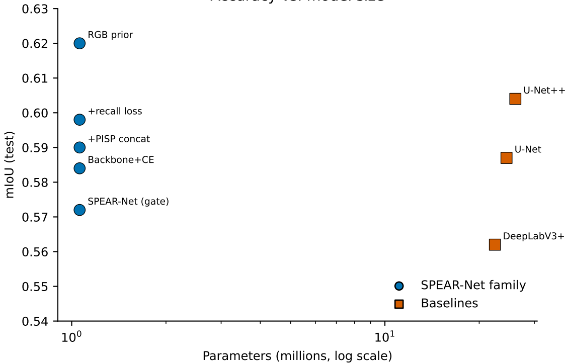
Accuracy vs. model size
