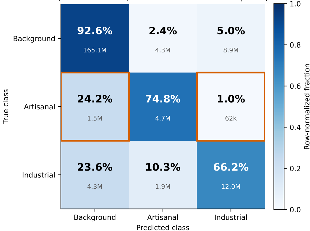
SPEAR-Net (gate): confusion matrix, test split (row-normalized; cell = share of true-class pixels)
