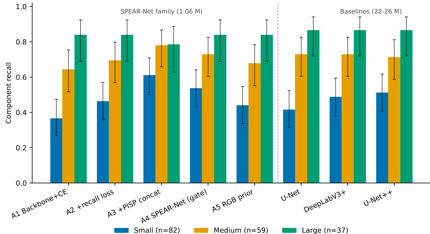
Area-stratified recall on the test split (95% Wilson CI)
