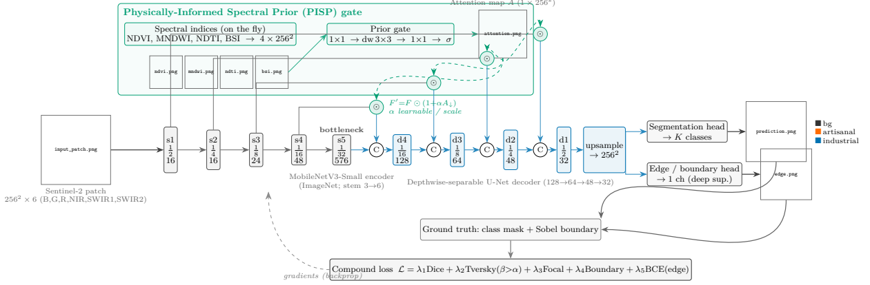
Figure 2: SPEAR-Net architecture. Four physically-informed spectral indices (NDVI, MNDWI, NDTI, BSI) are computed on the fly and passed through a small gate to a single spatial attention map A . In the depthwise-separable U-Net decoder each encoder skip is first gated by the attention, F' = F \odot (1 + \alpha A_{\downarrow}) with a per-scale learnable \alpha , and then concatenated ( \odot ) with the upsampled decoder feature; the deepest feature (s5) is the ungated bottleneck. A segmentation head and an auxiliary edge head (deep supervision) produce the outputs, and the compound loss compares them against the ground-truth mask and its Sobel boundary.
