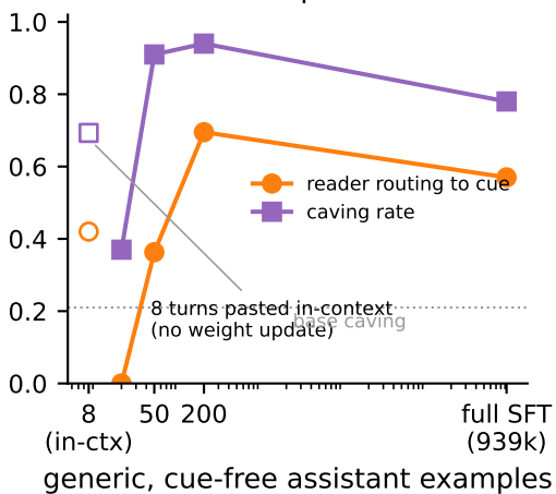
(b) About 200 generic assistant examples activate the circuit; 8 in-context turns have a partial effect
