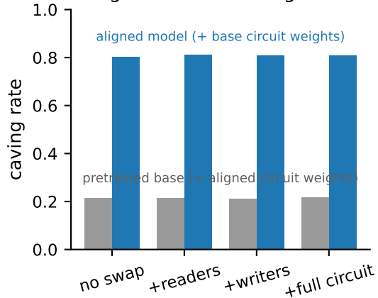
(a) Swapping circuit weights between base and aligned models changes nothing
