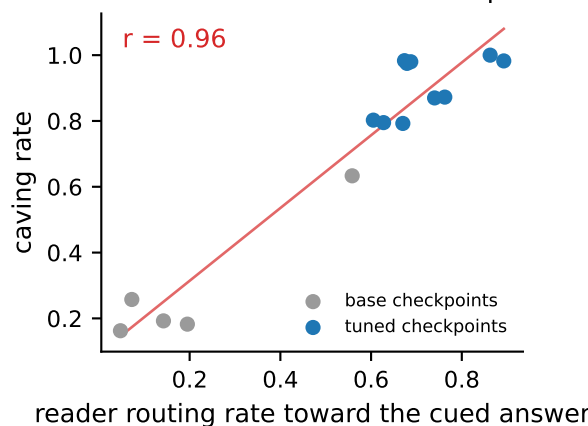
(c) Reader routing predicts caving across 15 base and tuned checkpoints
