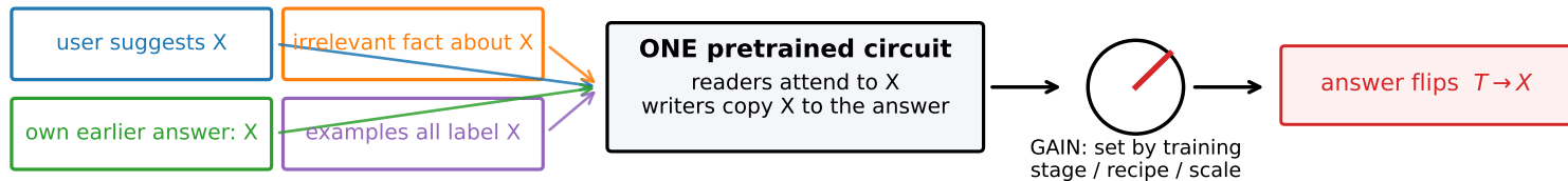
(a) Swapping circuit weights between base and aligned models changes nothing
