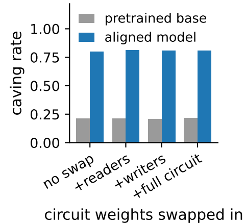
(a) Swapping circuit weights between base and aligned models changes nothing
