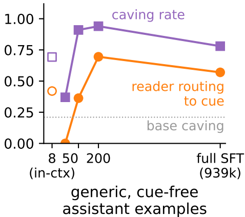
(b) About 200 generic assistant examples activate the circuit
