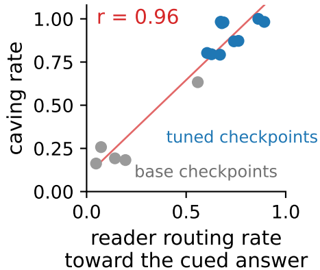
(c) Reader routing predicts caving across 15 checkpoints
