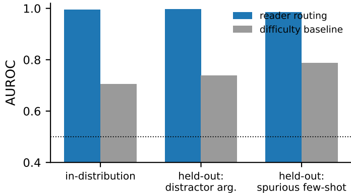
(a) Reader routing predicts caving before the answer (Gemma-2-2b)
