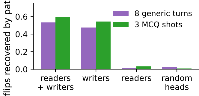
(b) In-context activation runs through the same circuit
