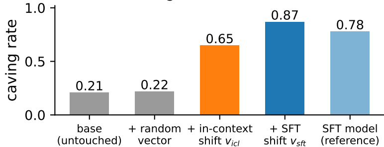
(a) Adding one activation direction to the base installs caving; random directions do not
