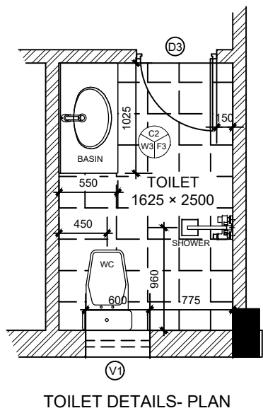
TOILET DETAILS- PLAN
