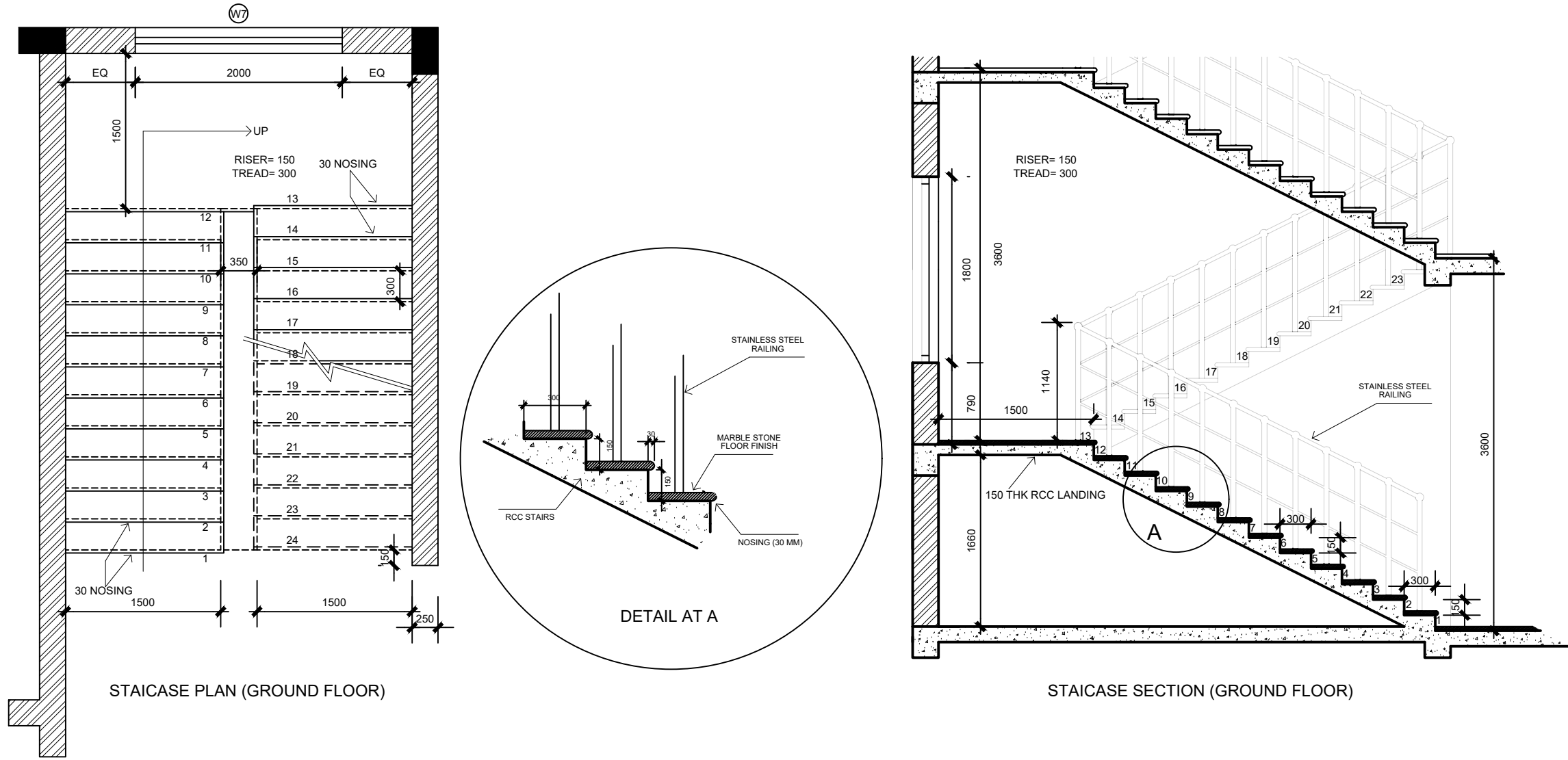
STAIRCASE PLAN (GROUND FLOOR)
