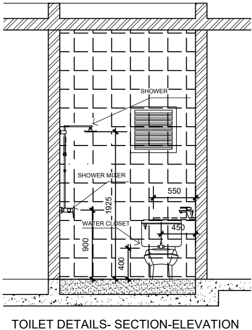
TOILET DETAILS- SECTION-ELEVATION
