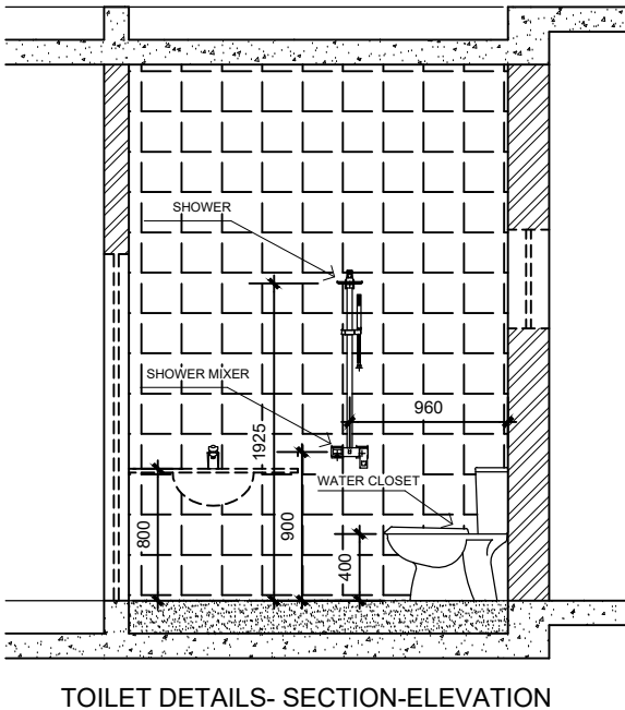
TOILET DETAILS- SECTION-ELEVATION
