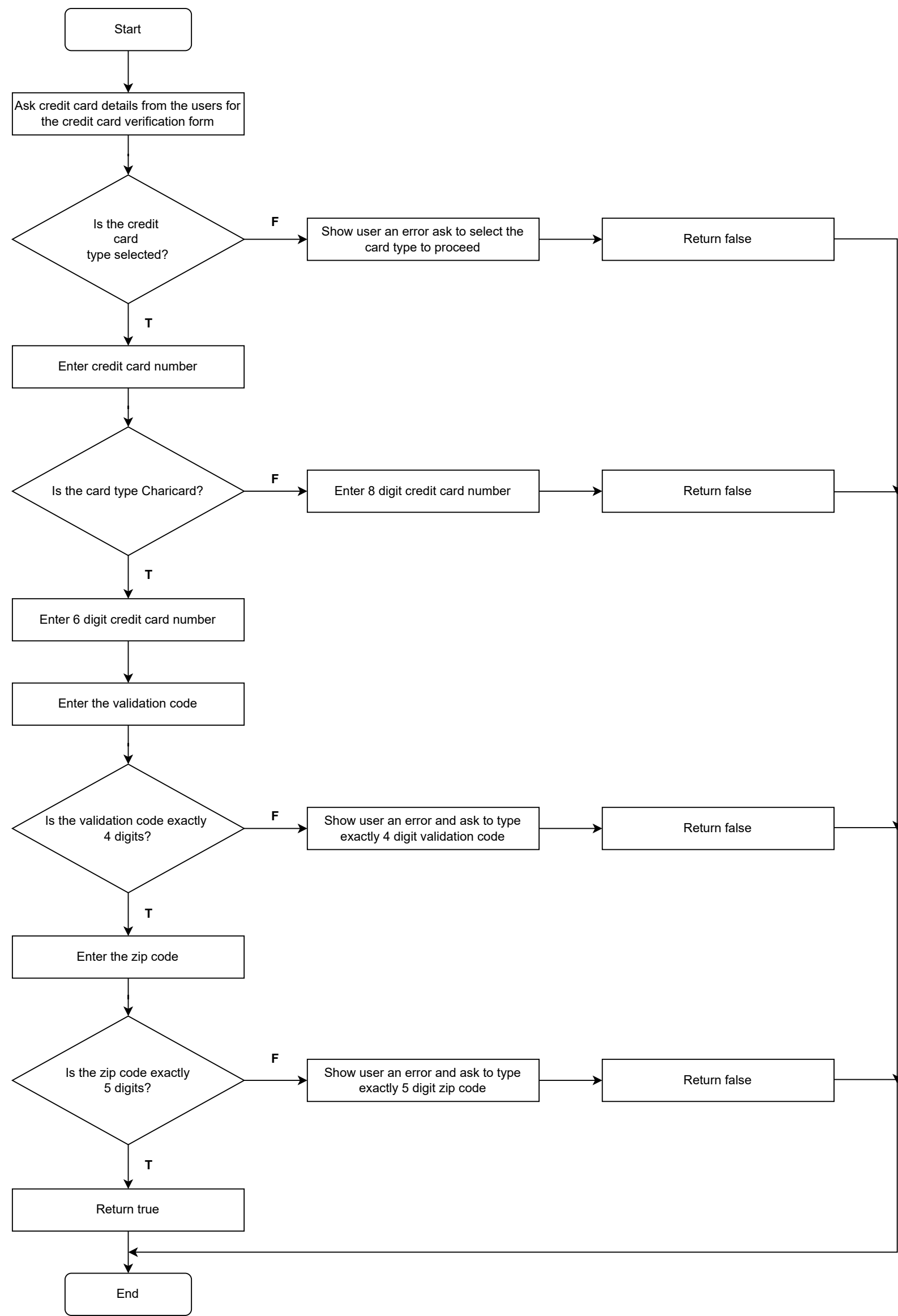
Flowchart of validateData
