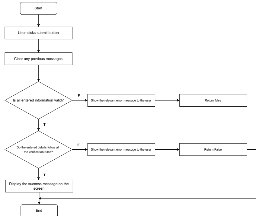
Flowchart of processForm
