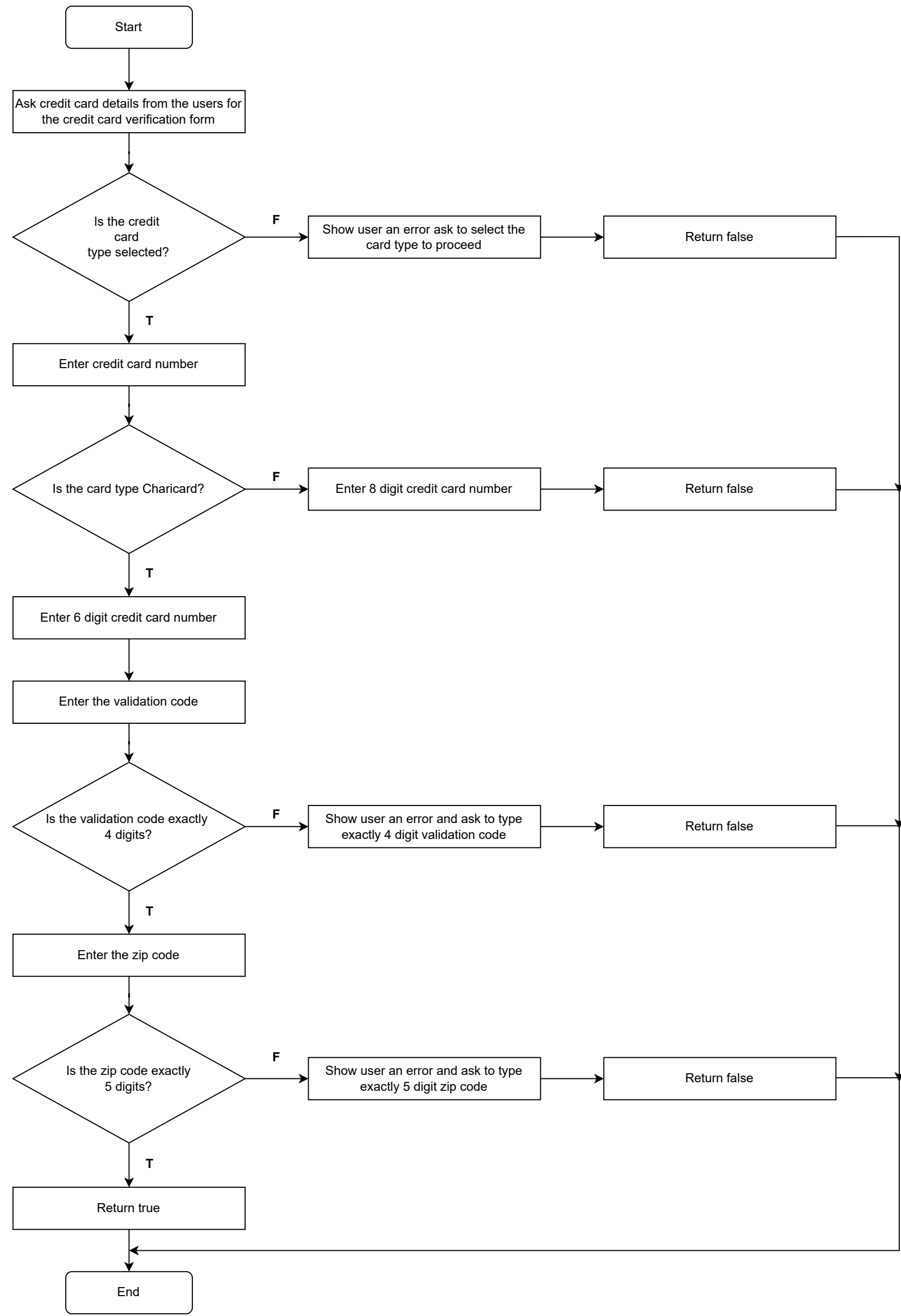
Flowchart of validateData
