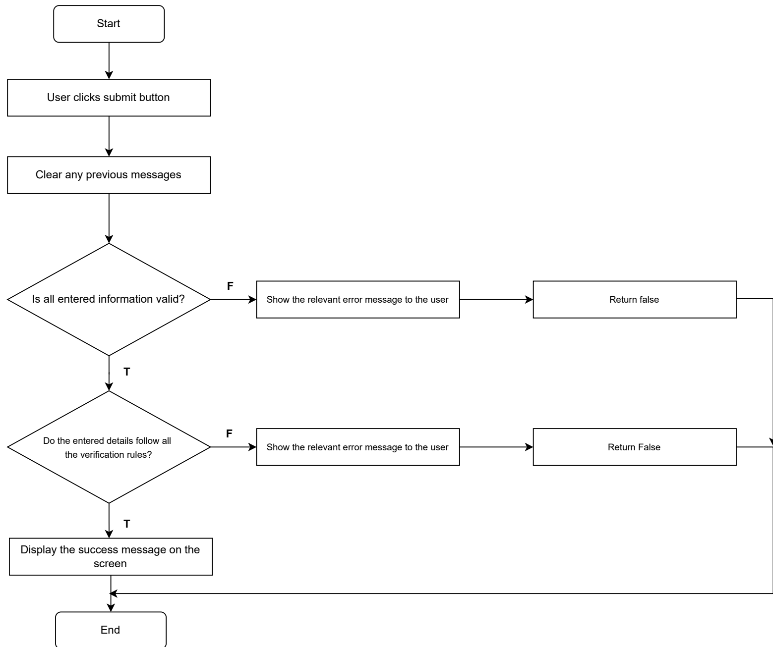
Flowchart of processForm
