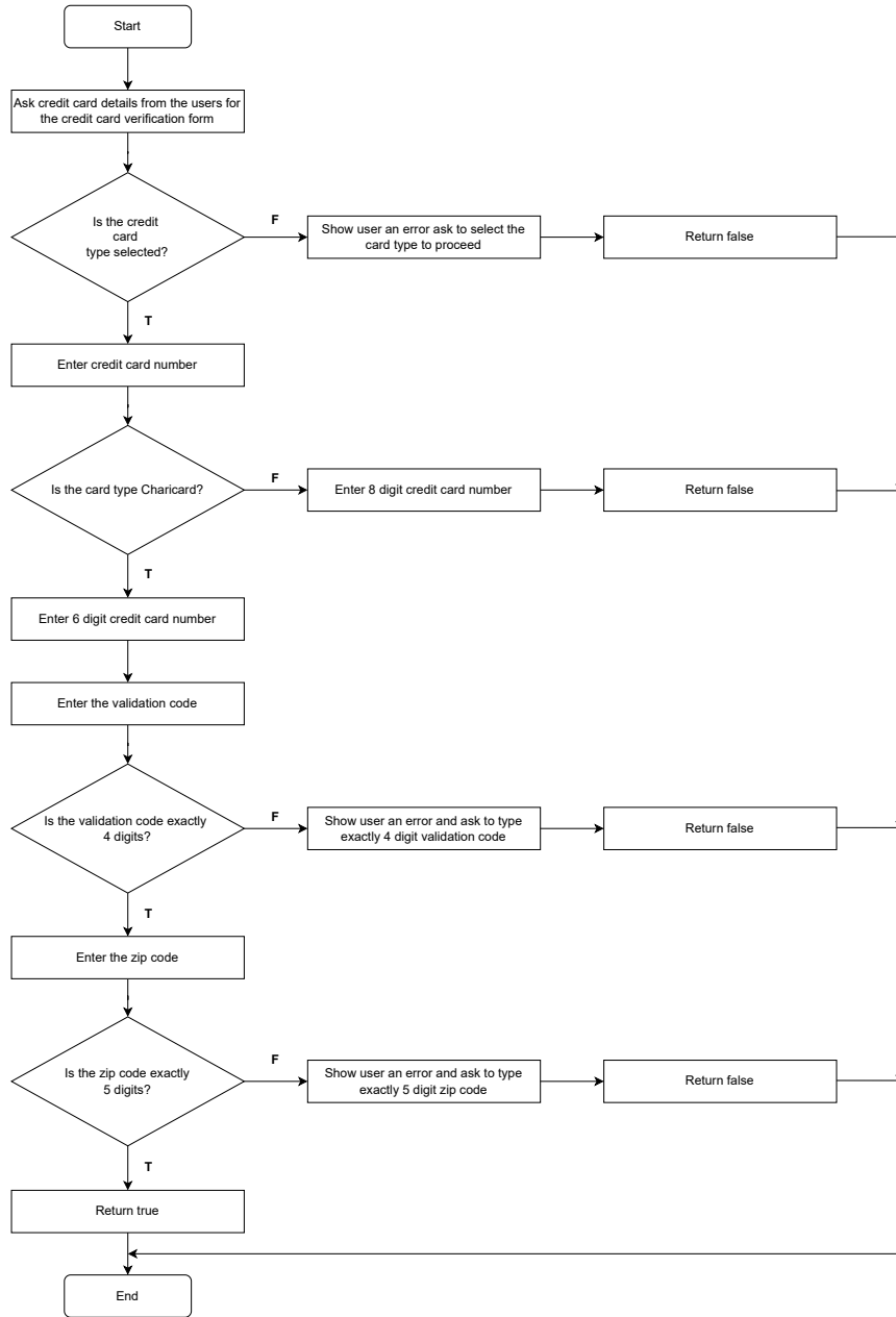
Flowchart of validateData
