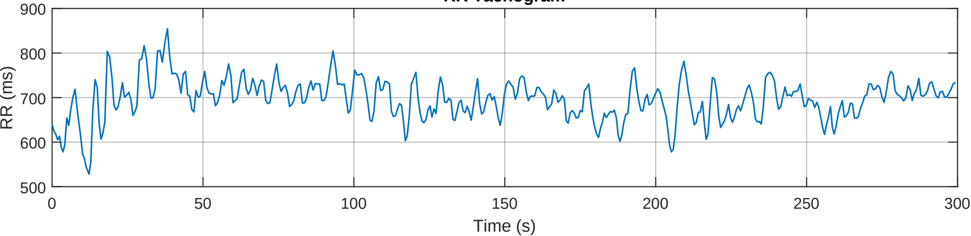
RR Tachogram
