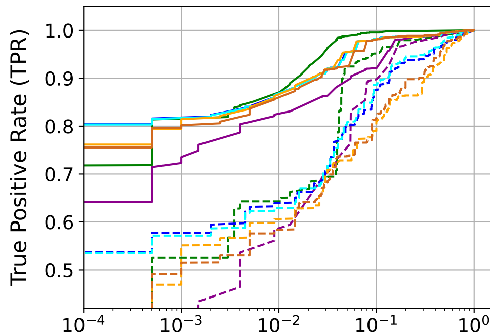
ModSec-Learn
