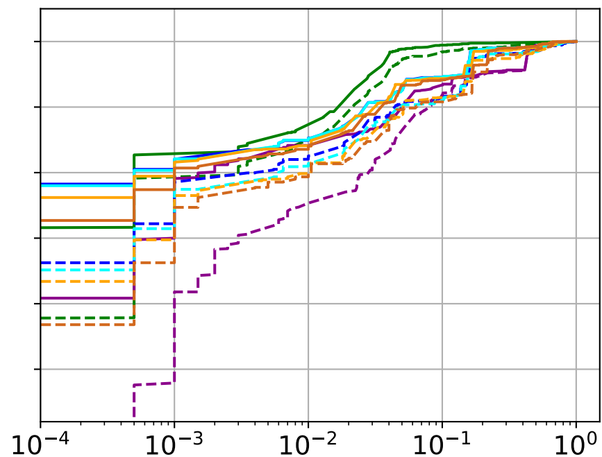
ModSec-AdvLearn
