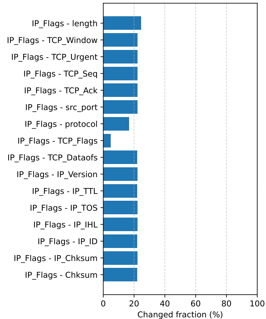
Random forest
