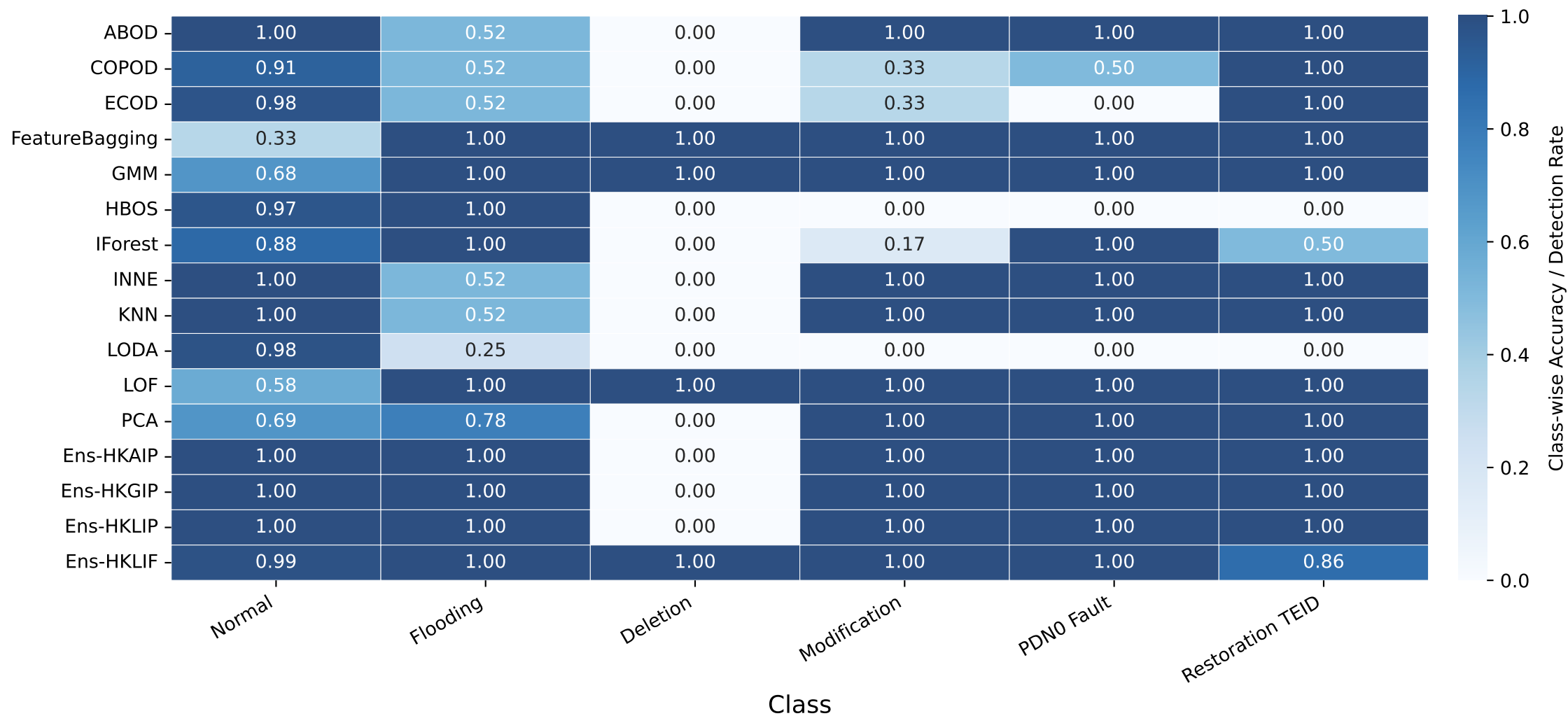
Class-wise Performance Heatmap (Normal + Attacks)
