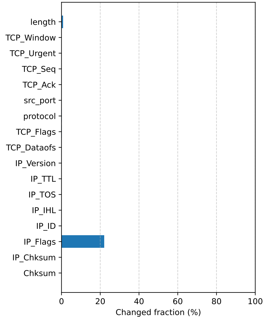
Random forest
