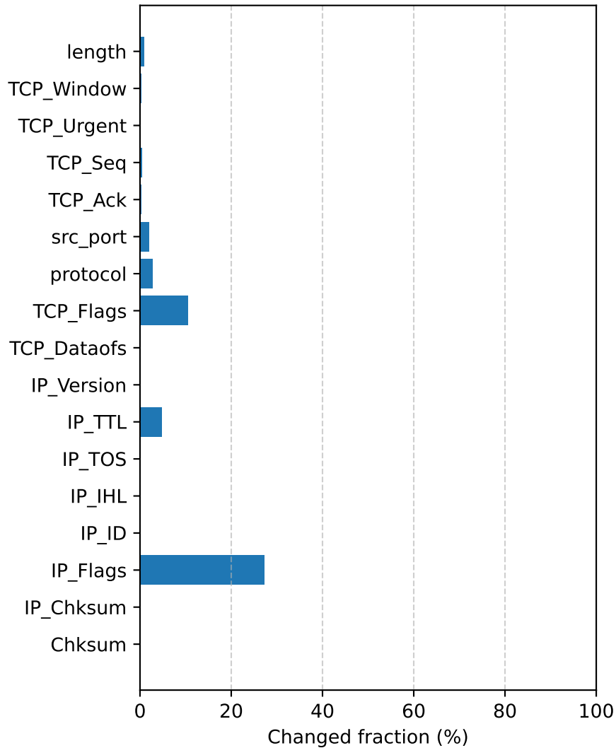
Isolation forest
