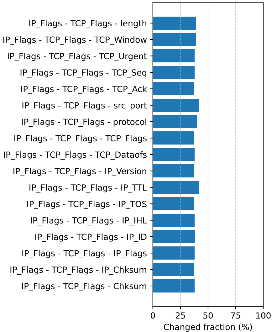
Isolation forest
