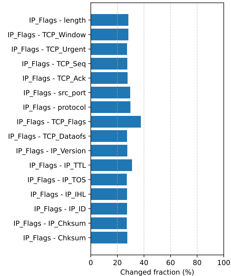
Isolation forest
