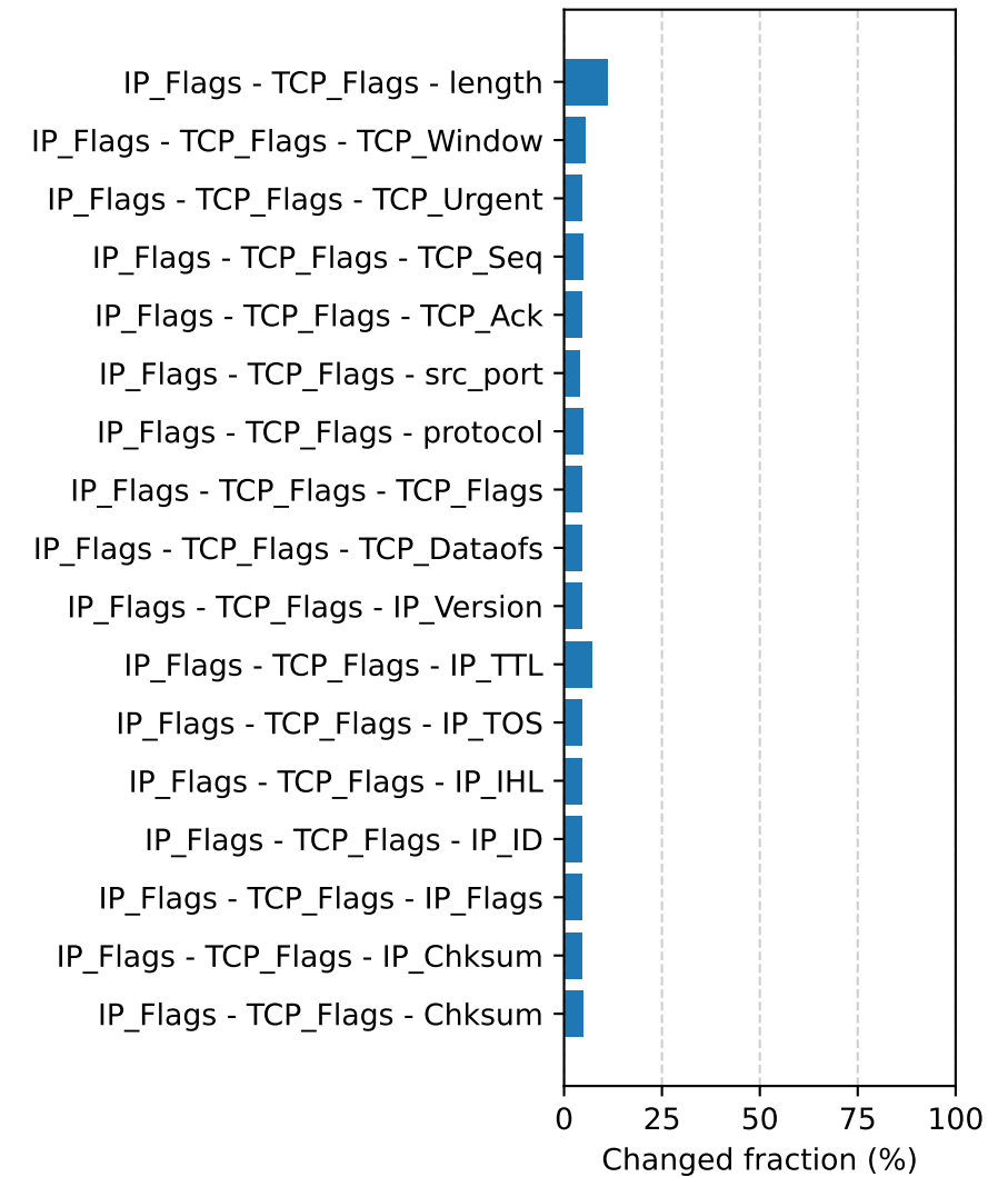
Random forest
