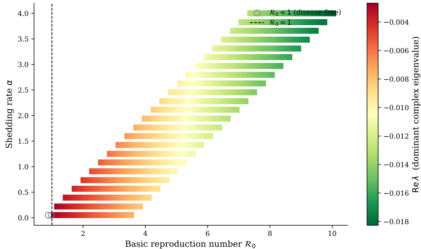
Stability of the endemic equilibrium across (\mathcal{R}_0, \alpha)
