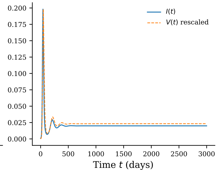
(c) Weakly damped: \mathcal{R}_0 = 5.27 , \alpha = 2.0
