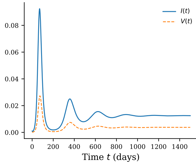
(b) Damped: \mathcal{R}_0 = 2.03 , \alpha = 0.10
