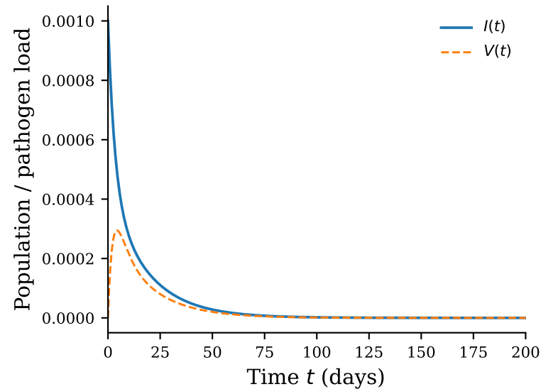
(a) Extinction: \mathcal{R}_0 = 0.56 < 1
