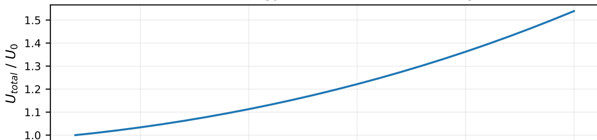
(b) Total EM energy (should increase during SHG)
