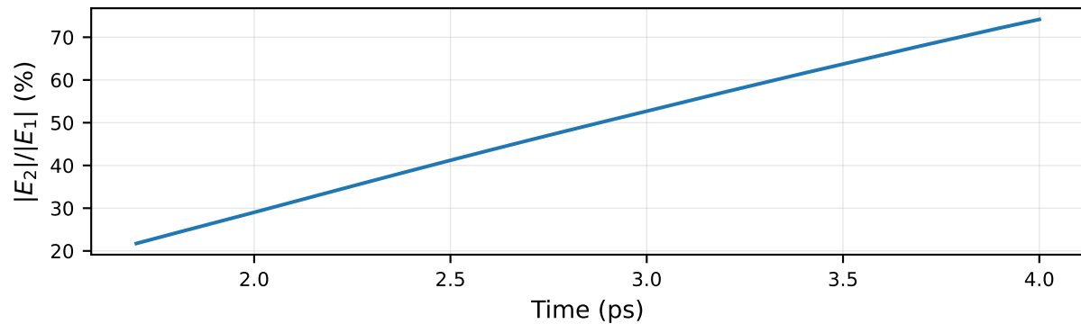
(c) Conversion efficiency
