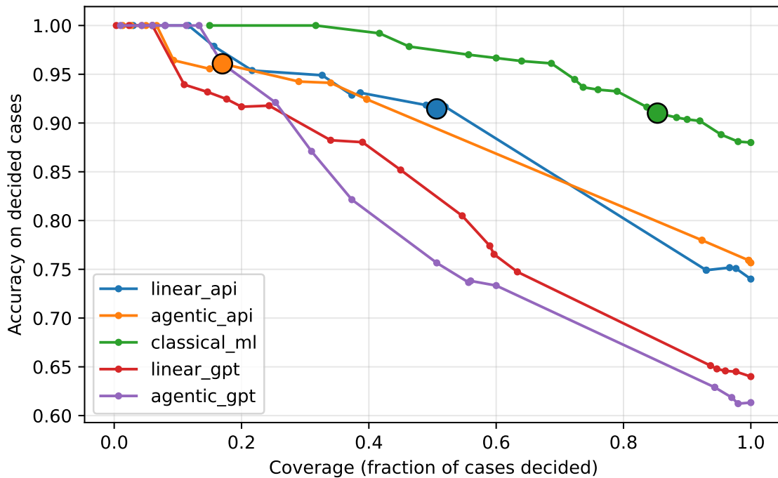
FIGURE 2. Full risk-coverage curves per arm, all five arms, with each Claude/ classical-ML arm's actual reported operating point marked (Section V-H's GPT arms omitted from the marked-point overlay for legibility; see Table 7 for their operating points). classical_ml's curve dominates every LLM arm from either model across nearly the entire coverage range, not merely at the specific chosen operating points—area under the risk-coverage curve (AURC) 0.0343 (classical_ml) vs. 0.1080 (linear_api) vs. 0.1117 (agentic_api) vs. 0.1850 (linear_gpt) vs. 0.2046 (agentic_gpt); lower is better.
