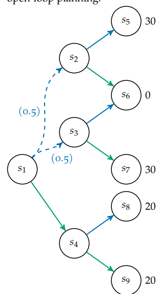
Example 9.9. Suboptimality of open-loop planning.
