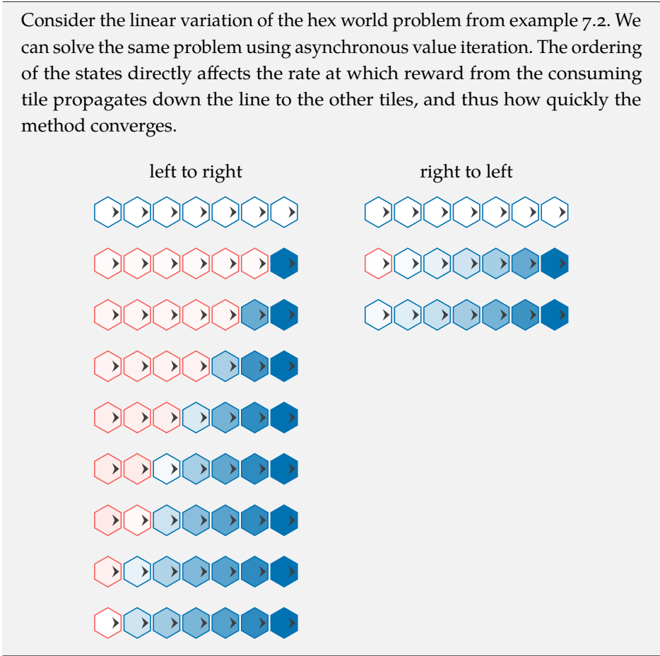
Example 7.3. The effect of the state ordering on convergence of asynchronous value iteration. In this case, evaluating right to left allows convergence to occur in far fewer iterations.
