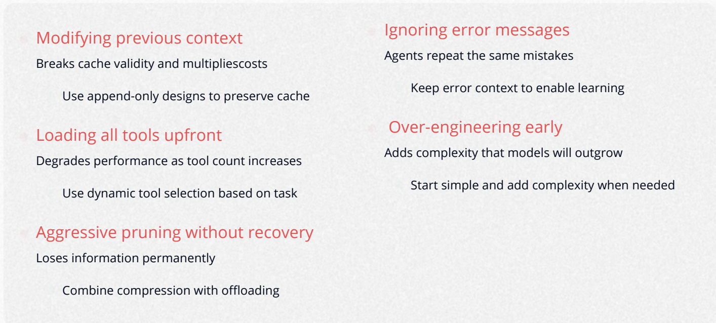
FIGURE 4.8 Common context engineering mistakes and corrections
