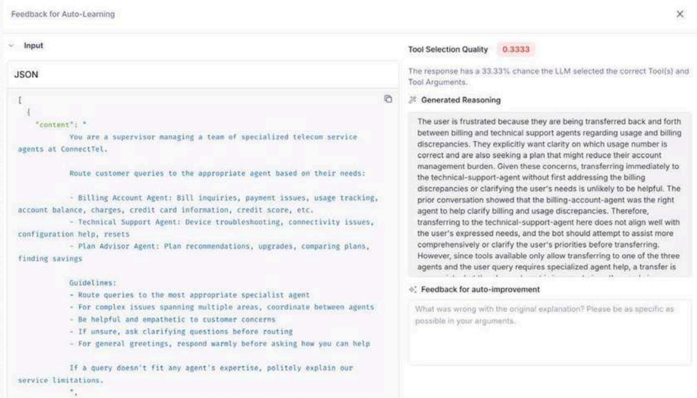
FIGURE 5.7 Metric Explanations
