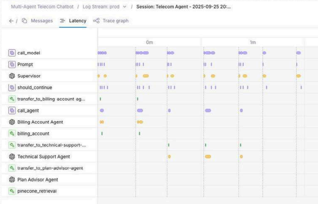
FIGURE 5.8 Timeline View
