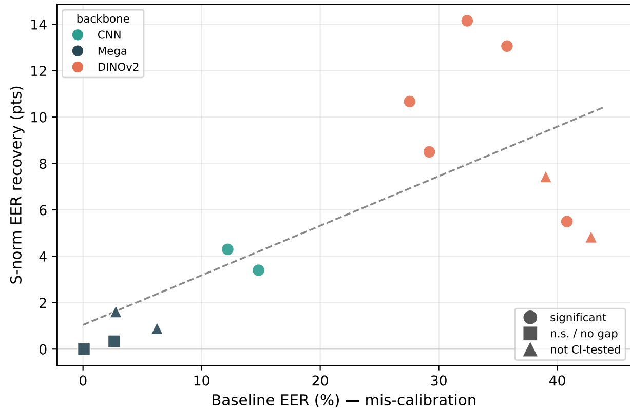
Calibration recovery scales with baseline mis-calibration
