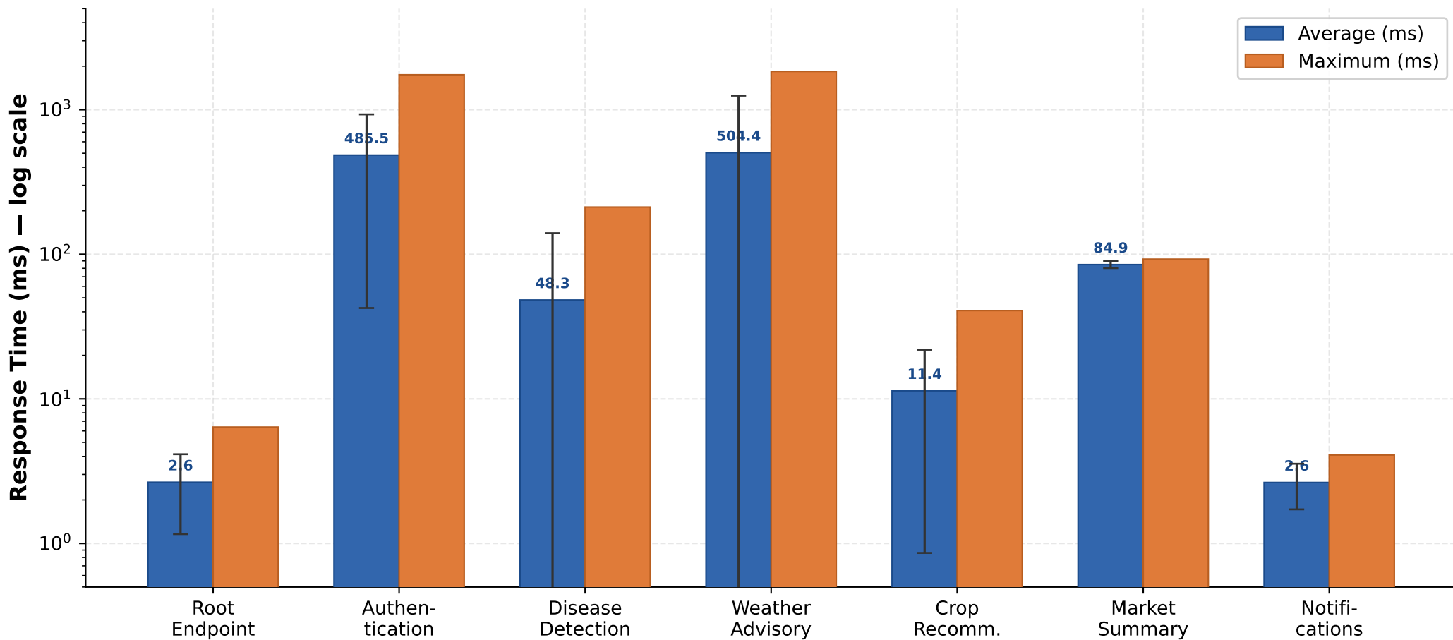
Fig. 2: API Response Time Benchmarks Across All ALIP Modules (Error bars indicate standard deviation)
