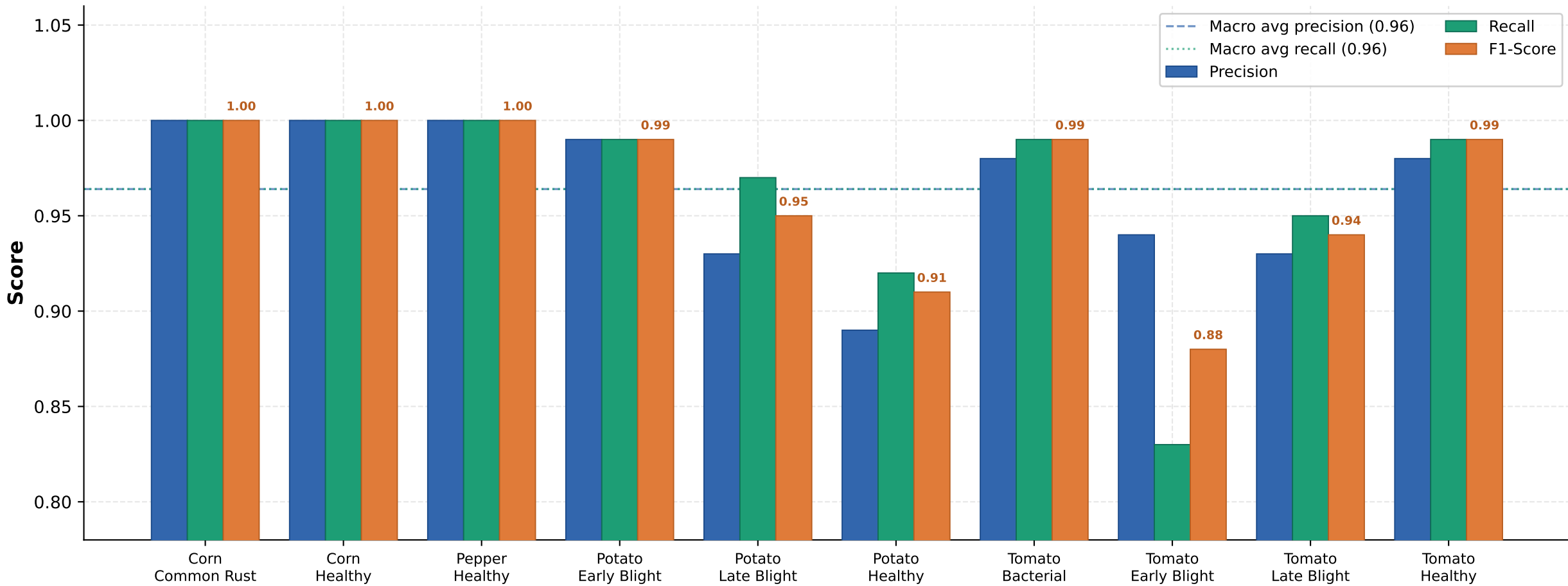
Fig. 3: Per-Class Classification Performance (Precision, Recall, F1-Score)
