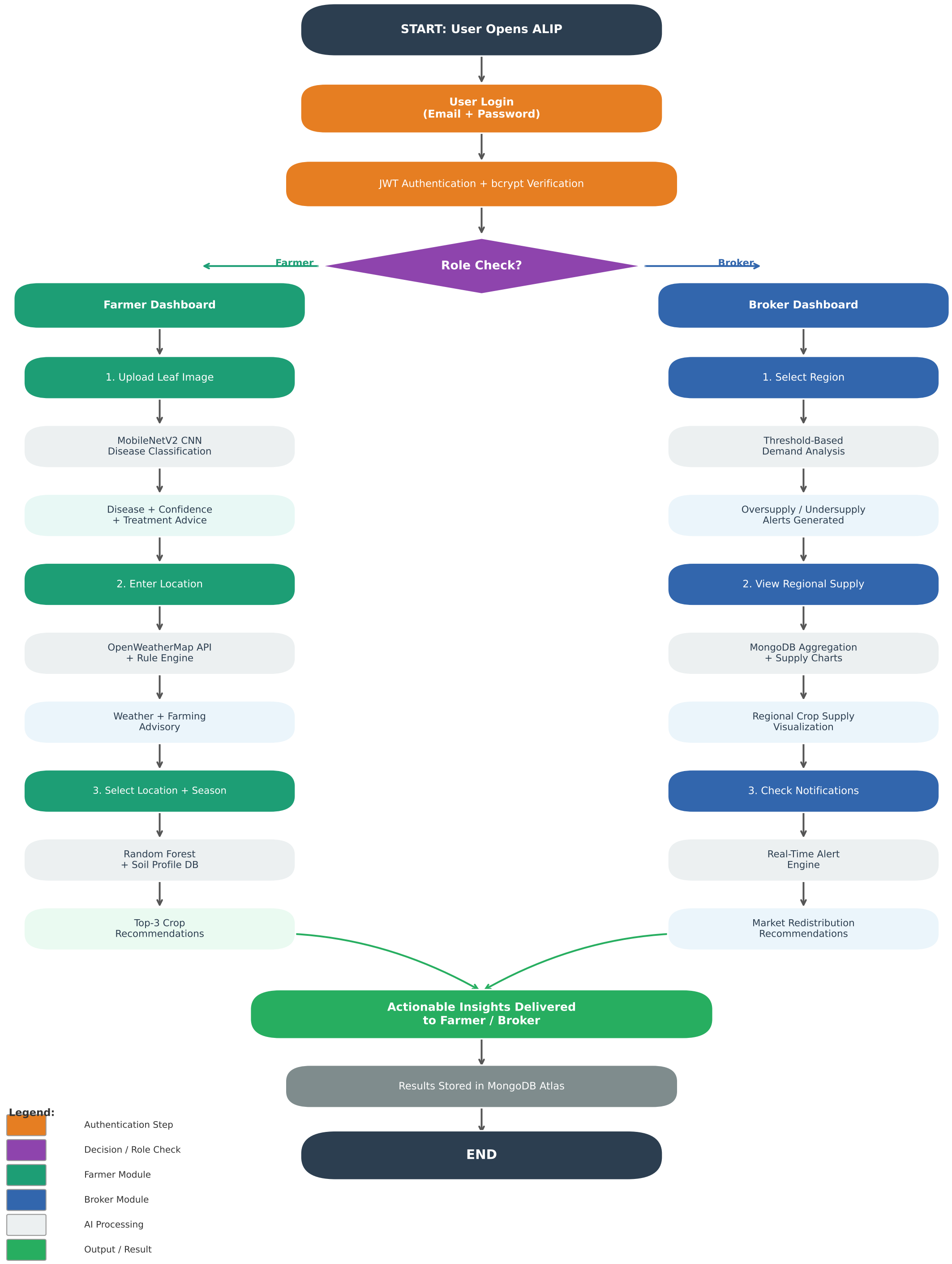
Fig. 5: End-to-End Operational Workflow of the ALIP System — From Authentication to Insight Delivery
