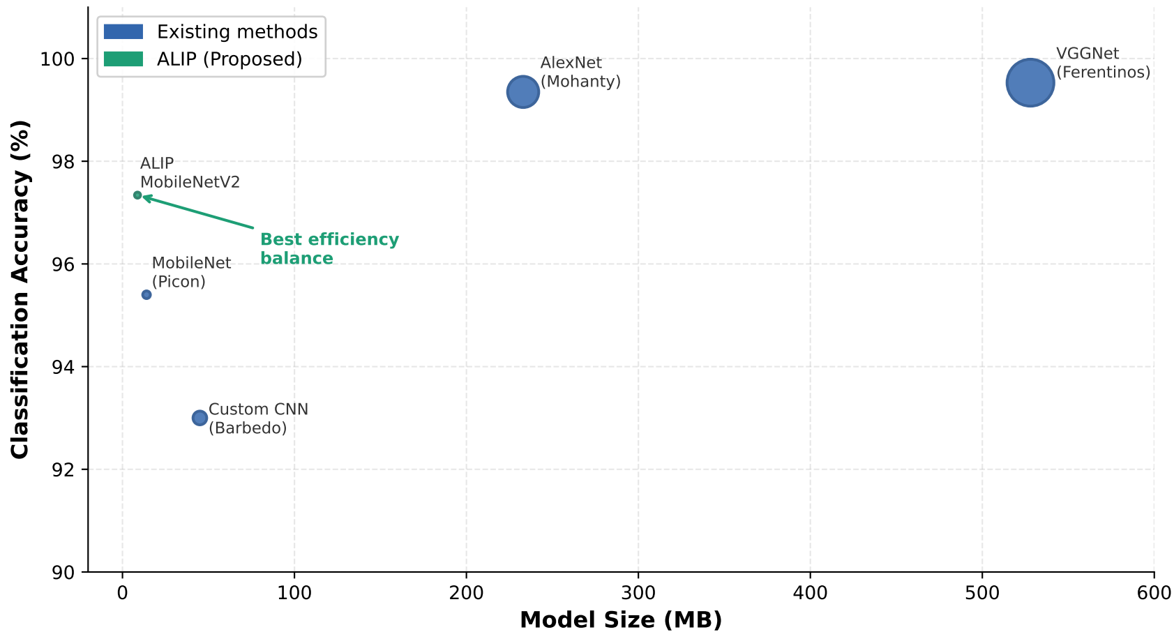
Fig. 6: Model Size vs. Classification Accuracy (Bubble size proportional to model size)
