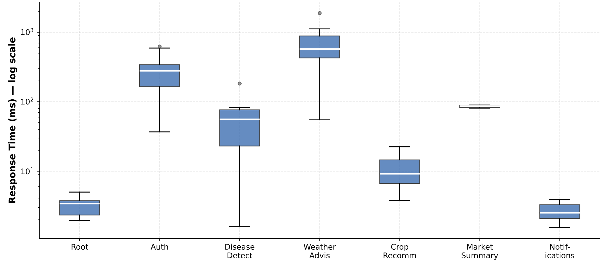
Fig. 7: Response Time Distribution Across ALIP Modules (10 requests per module, log scale)
