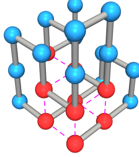
Figure 2.1: Illustration of the 3D HP lattice model showing a short self-avoiding walk. Hydrophobic residues (H) are shown in red, polar residues (P) in blue. Dotted magenta lines indicate valid non-consecutive H-H contacts that contribute to the energy function, this contact has energy -9 \epsilon_{HH} .
