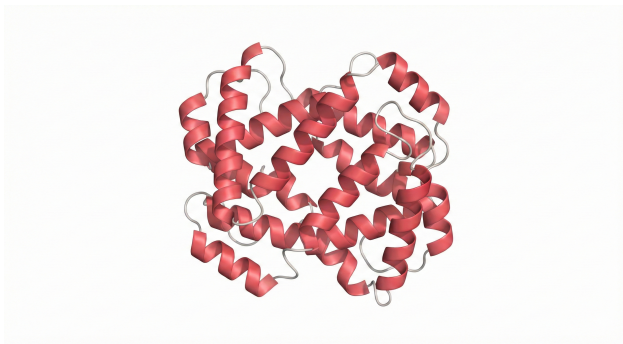
Figure 1.1: Three-dimensional structure of the haemoglobin beta subunit - figure created by author using Nano Banana
