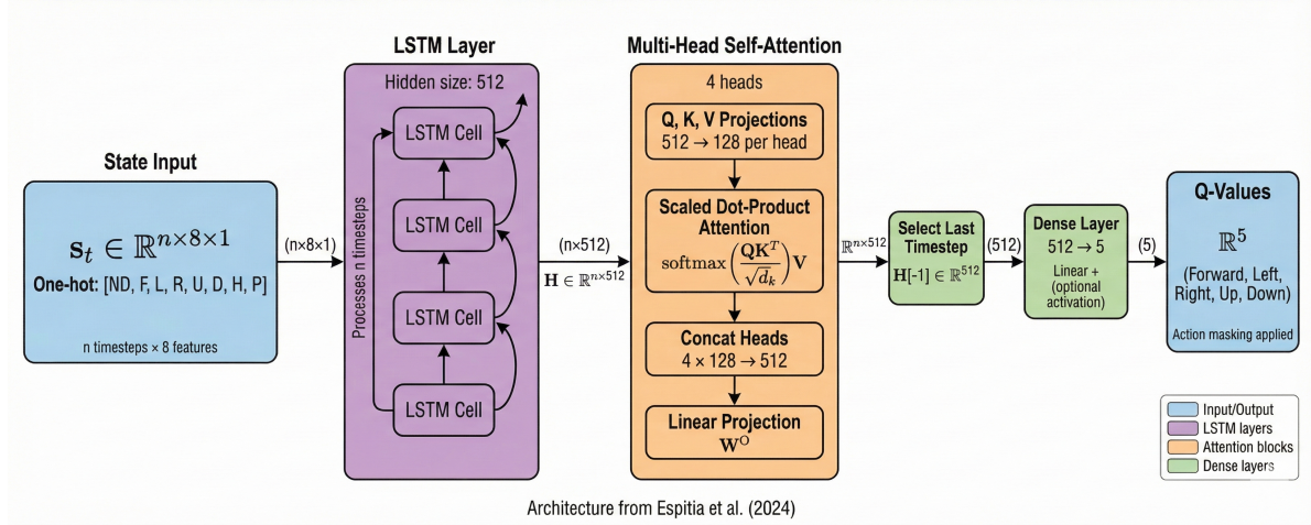
Figure 2.2: LSTM-A architecture from Espitia et al. (2024). The state input (n, 8, 1) is processed through LSTM cells (hidden size 512) followed by 4-head multi-head self-attention. The last timestep of the attention output is mapped to Q-values for the 5 placement actions through a dense layer. Figure created by the author using Nano Banana.
