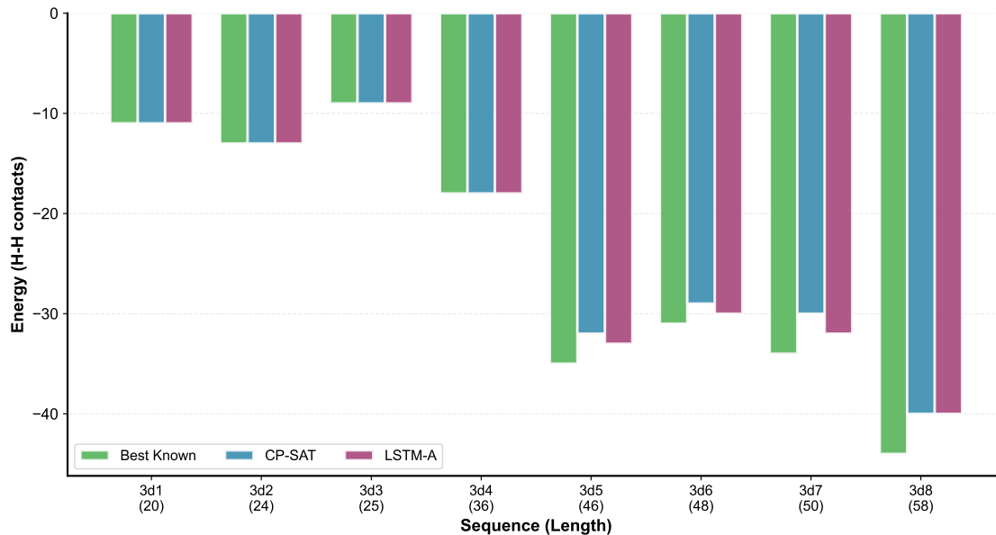
Figure 3.2: Solution quality comparison across benchmark sequences. Both methods achieve optimal solutions for sequences up to length 36 (3d1–3d4). Performance degrades gracefully on longer sequences, with gaps of 2–5 contacts from best-known values.
