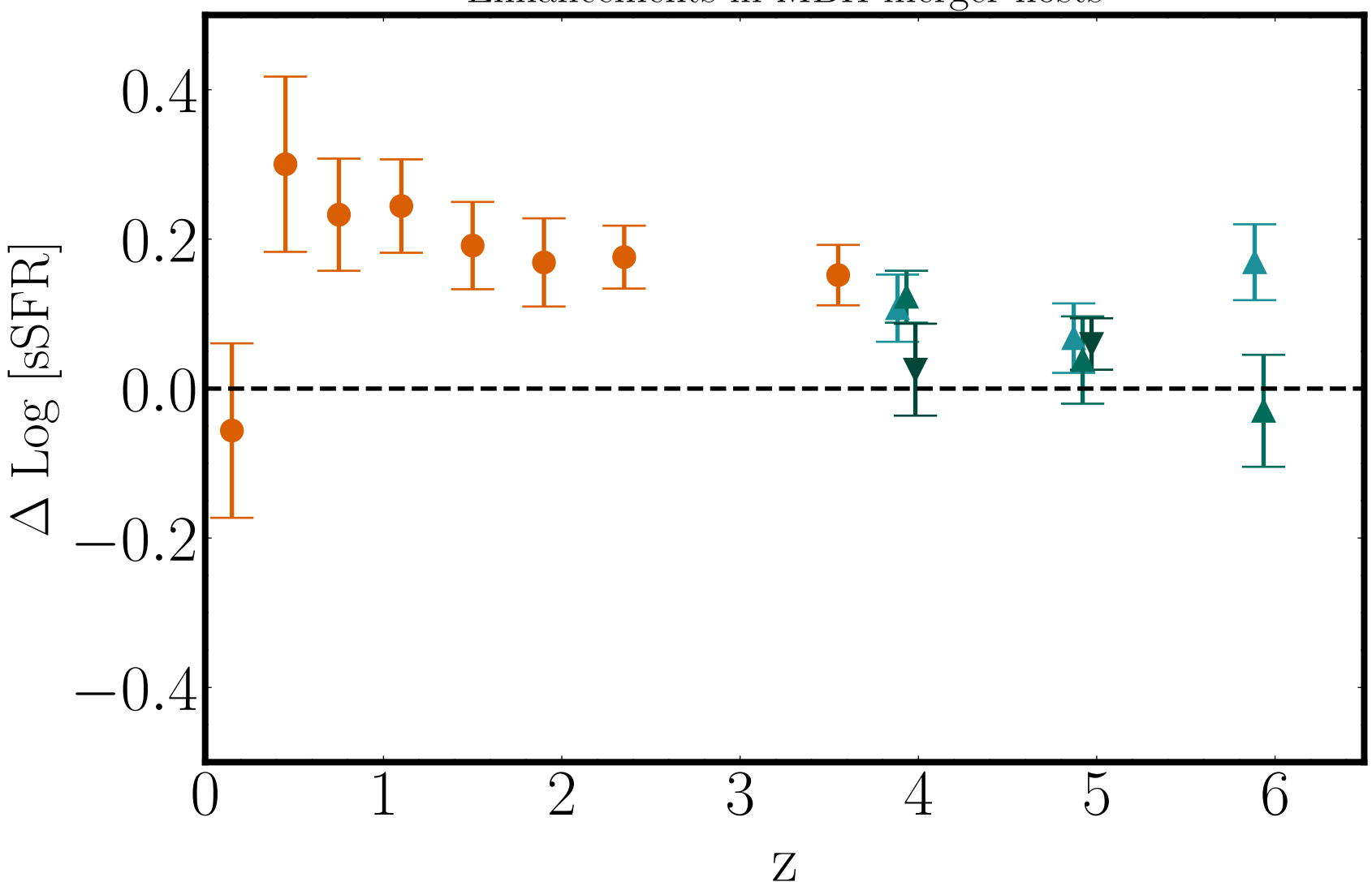
Enhancements in MBH merger hosts
