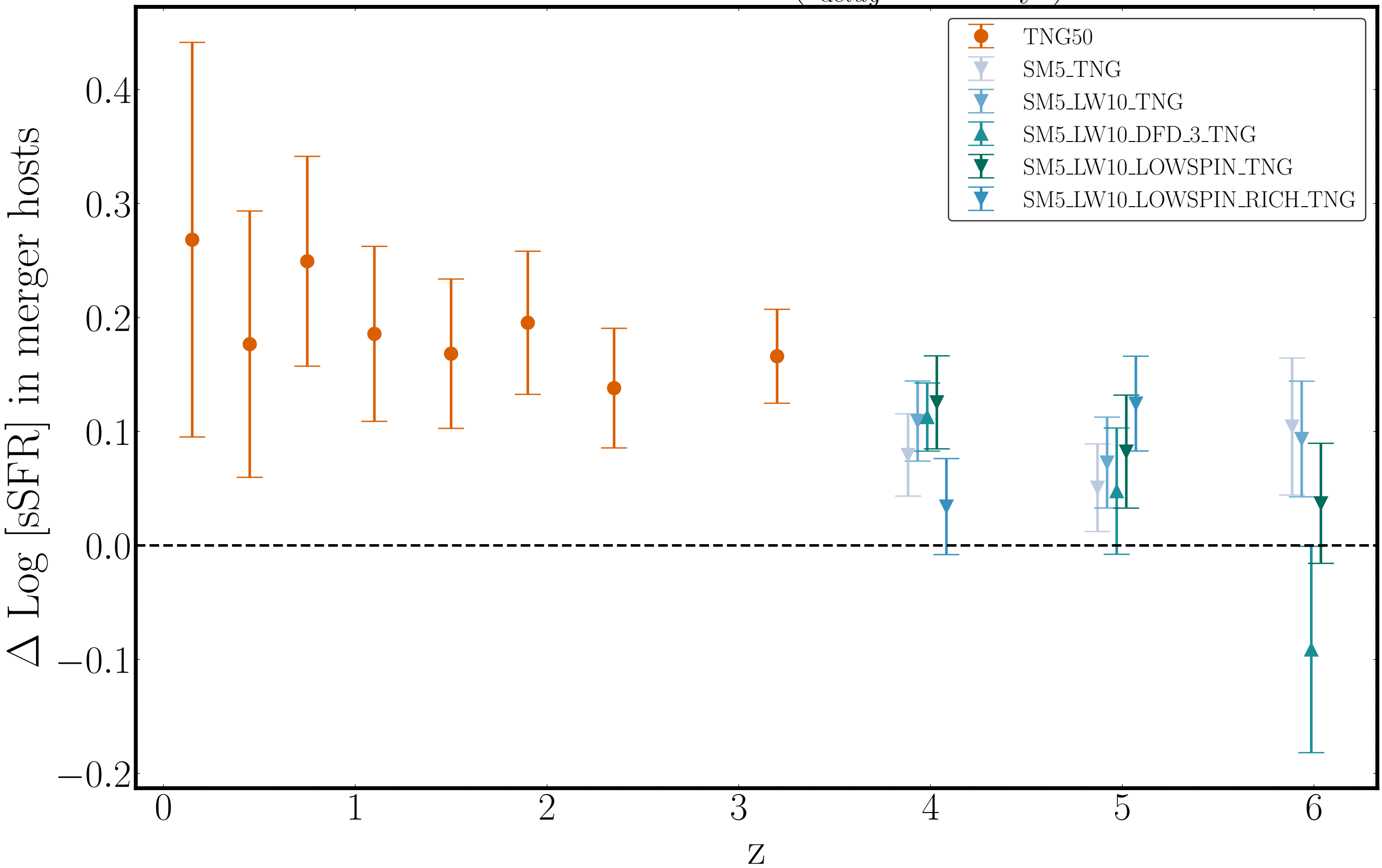
TNG50 + BRAHMA ( t_{\text{delay}} < 0.5 Gyr)
