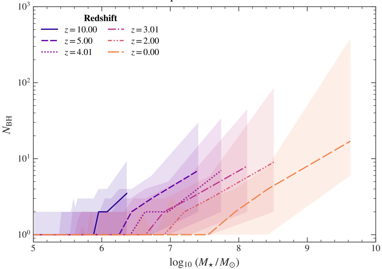
Black-hole occupation versus host stellar mass
