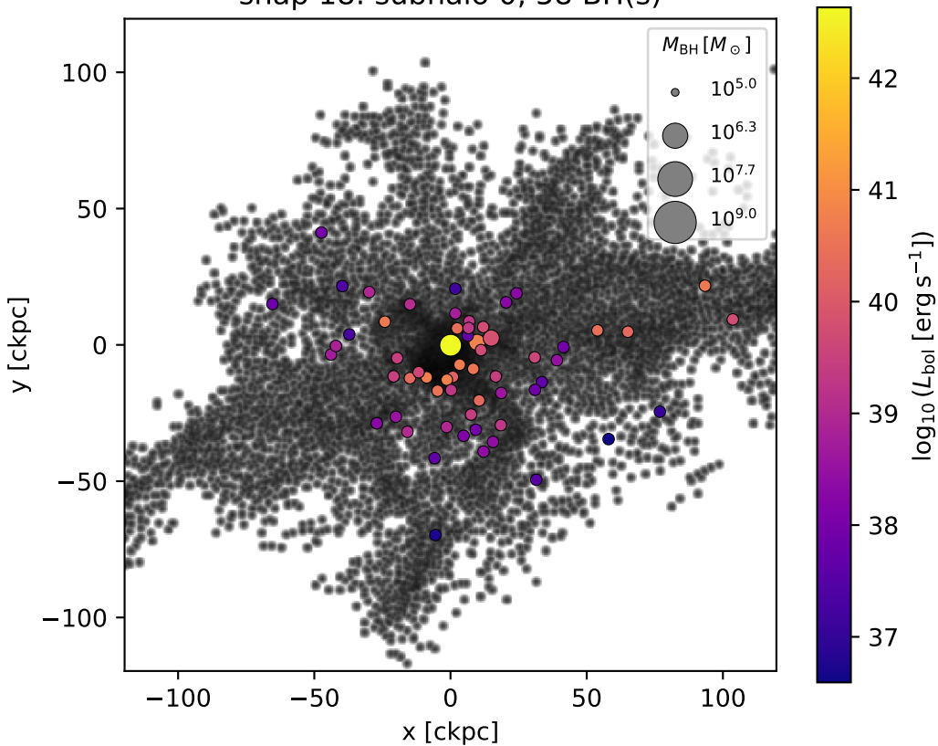
snap 18: subhalo 0, 58 BH(s)
