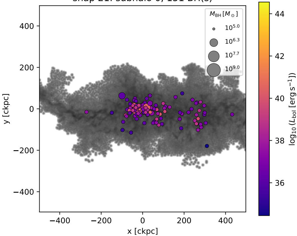
snap 21: subhalo 0, 151 BH(s)
