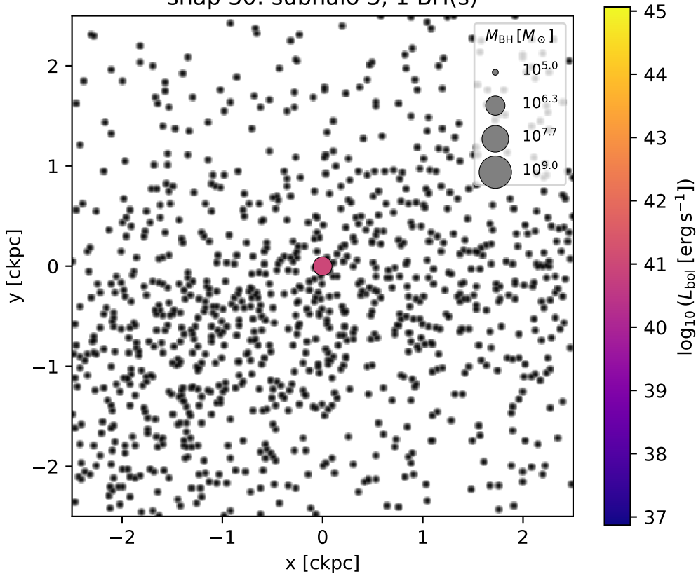
snap 30: subhalo 3, 1 BH(s)
