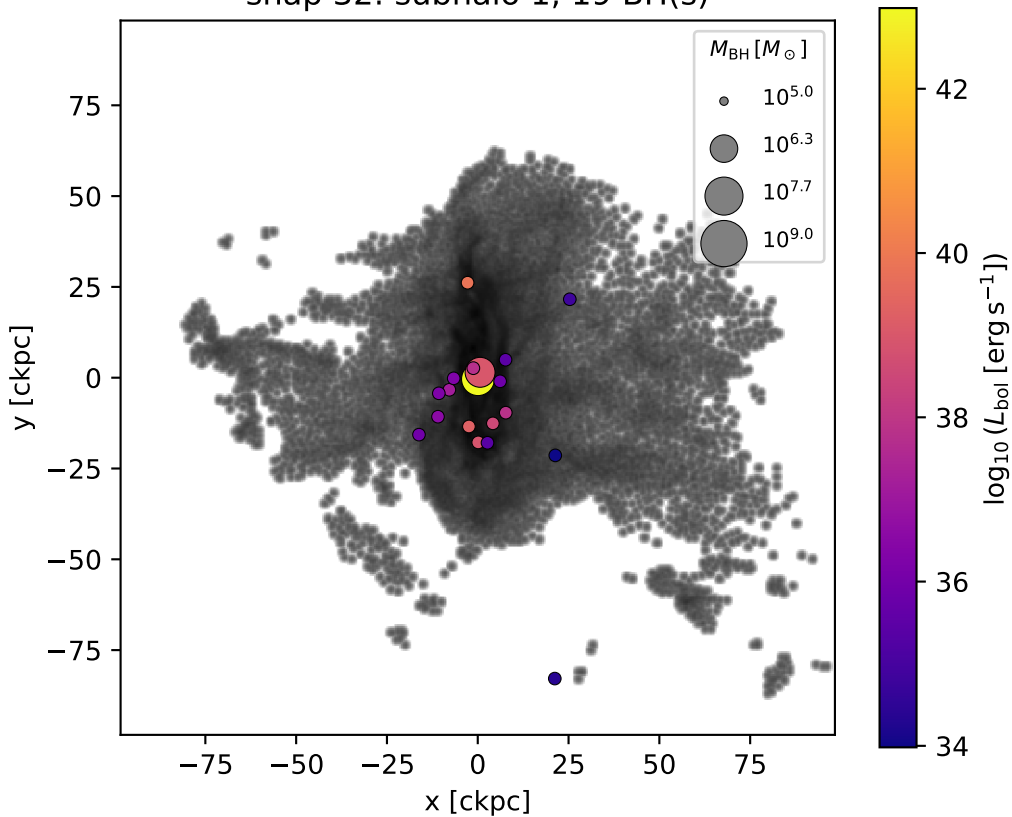
snap 32: subhalo 1, 19 BH(s)
