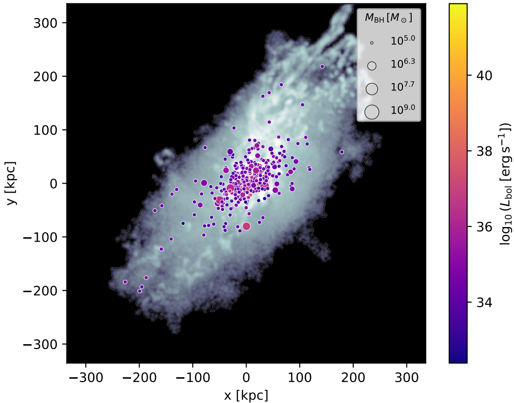
z = 0.50 : subhalo 1, 455 BH(s)
