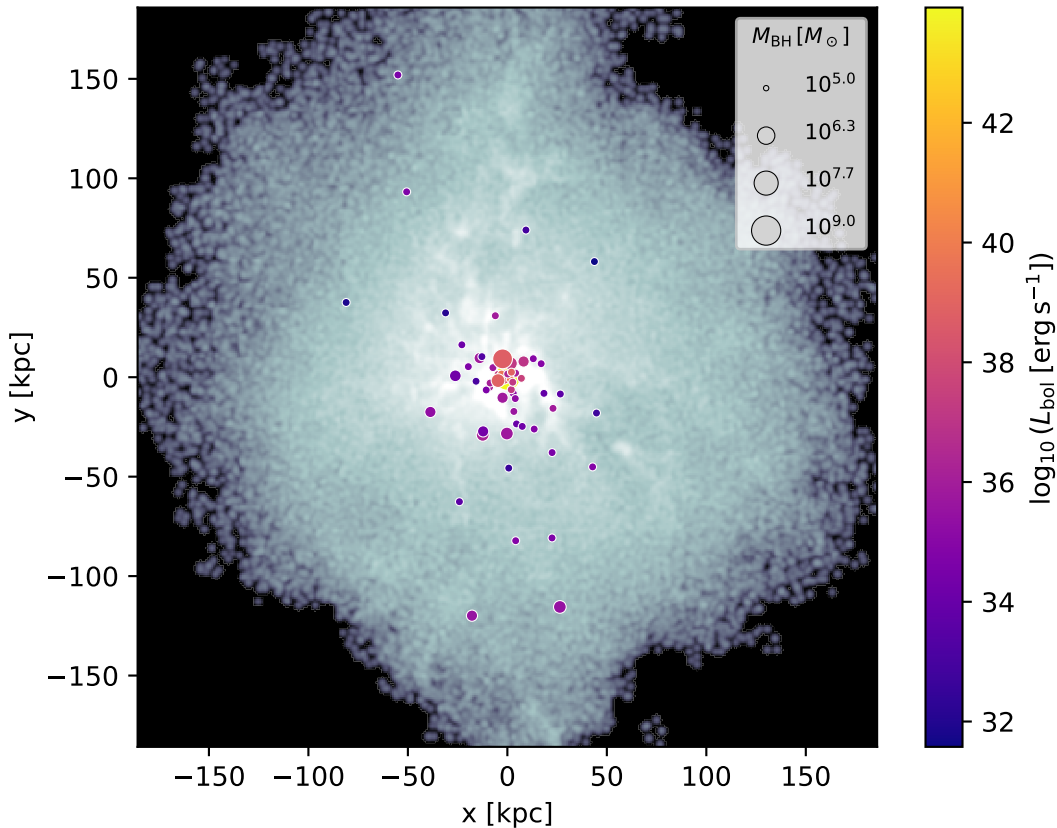
z = 0.00 : subhalo 6247, 60 BH(s)
