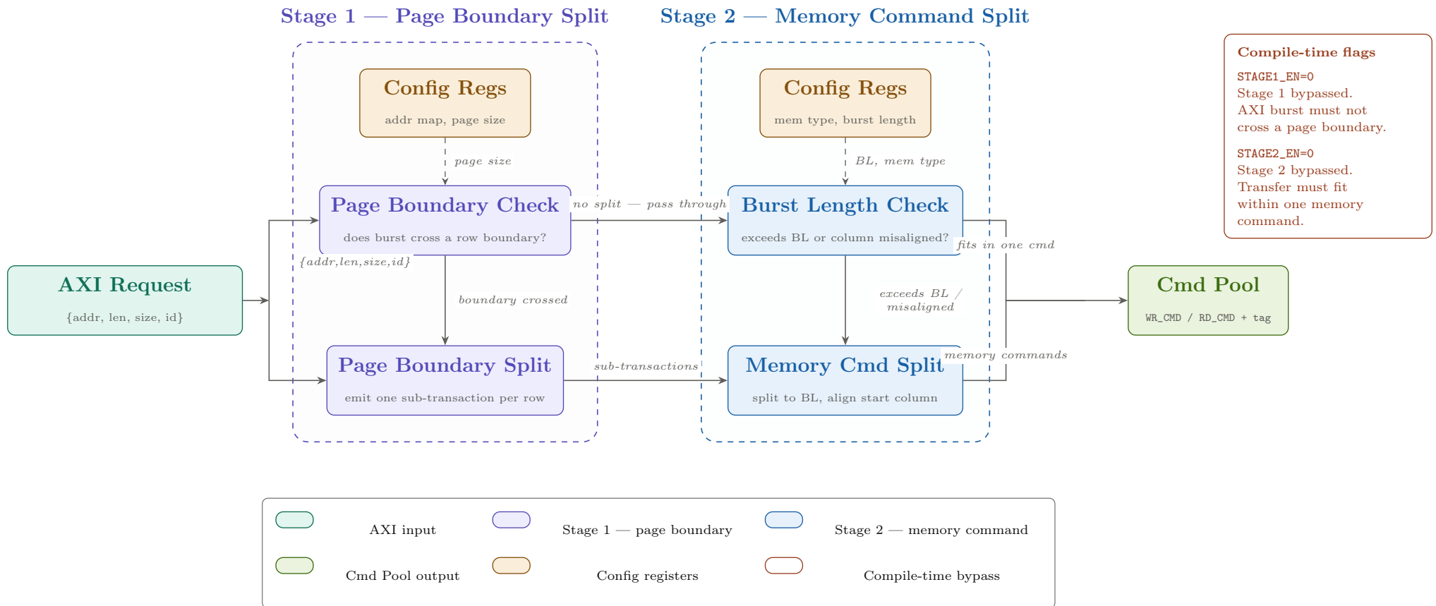
Figure 1: Burst Splitter internal pipeline. Stage 1 splits an AXI Request at row (page) boundaries into linear transactions each confined to a single row. Stage 2 divides each into memory commands sized to the configured burst length and aligned to the start column address. Both stages are individually enabled or disabled at compile time.
