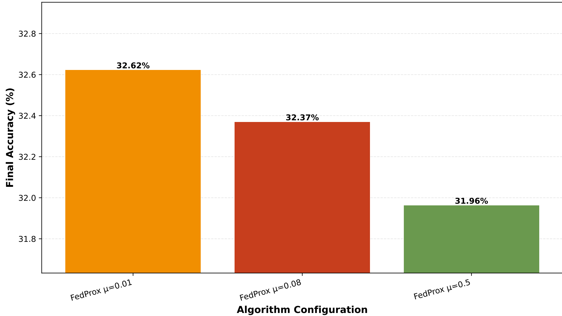
CIFAR-100 Brittleness Study: Final Accuracy Comparison
