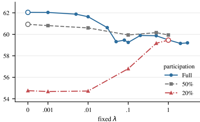
B CIFAR pathological
