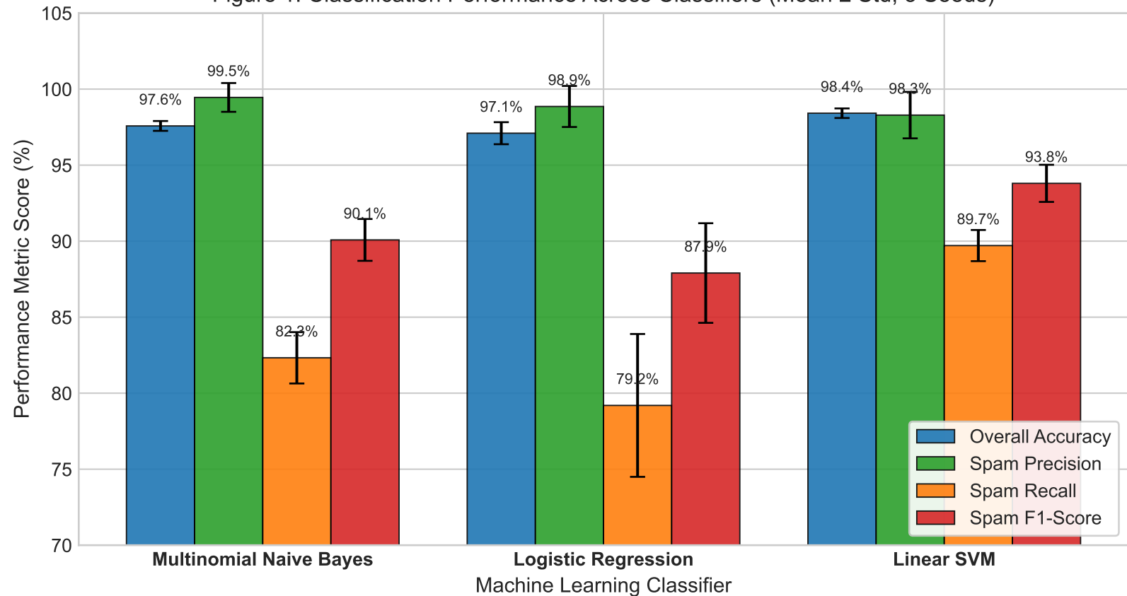
Figure 1: Classification Performance Across Classifiers (Mean \pm Std, 3 Seeds)
