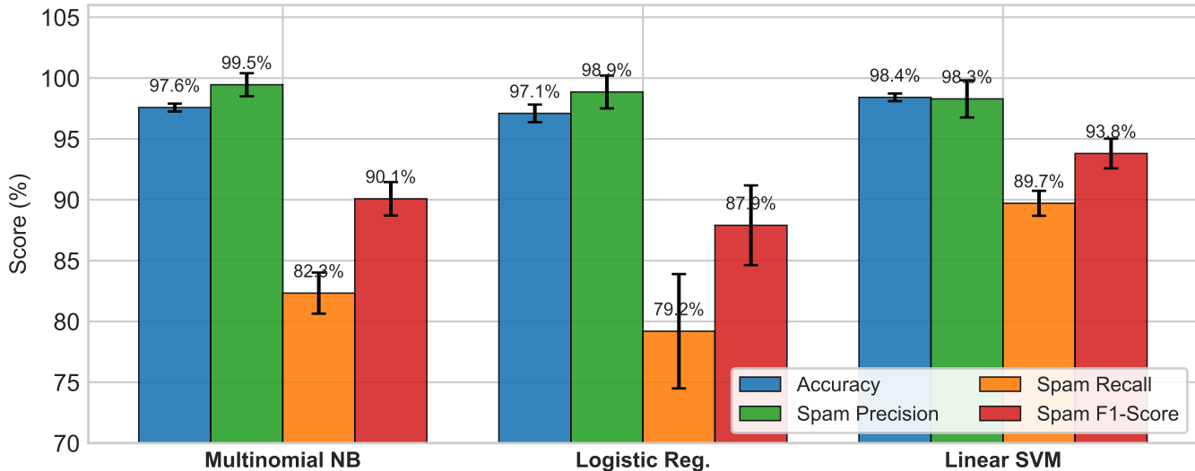
Figure 1: Classifier Performance Comparison (Mean \pm Std, 3 Seeds)
