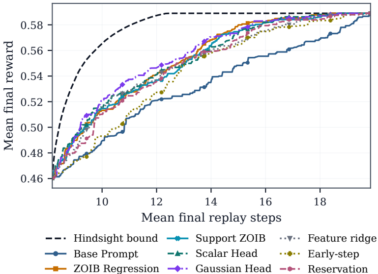
WebShop: Absolute reward
