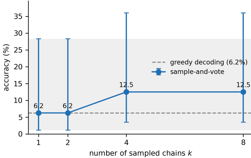
Figure 4: Accuracy of Qwen2.5-0.5B-Instruct on GSM8K as a function of sampled chains k (majority vote), versus the greedy baseline (dashed). Error bars and the gray band are Wilson 95% intervals. Data and code: code/exp4_self_consistency.py .
