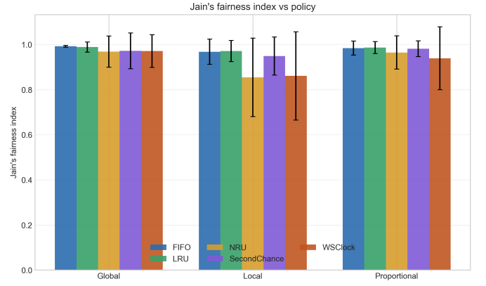
Fig. 3. Jain's fairness index vs. allocation policy in the cleaned canonical aggregate.
